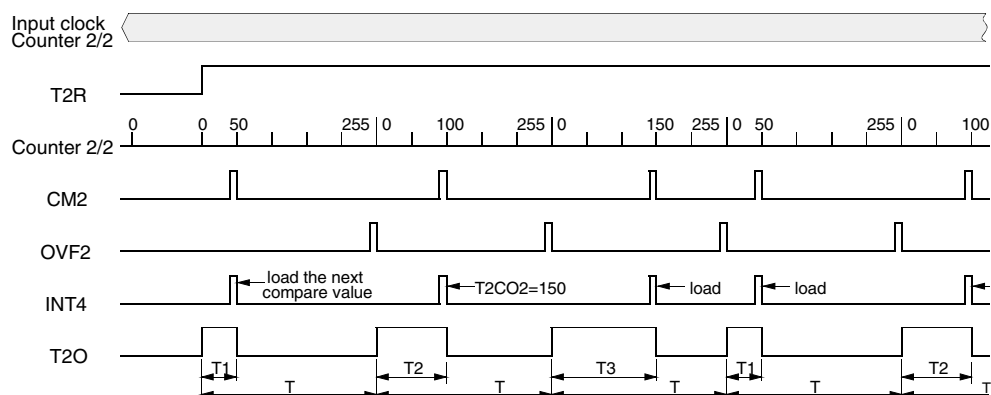
Figure 38. PWM Modulation
