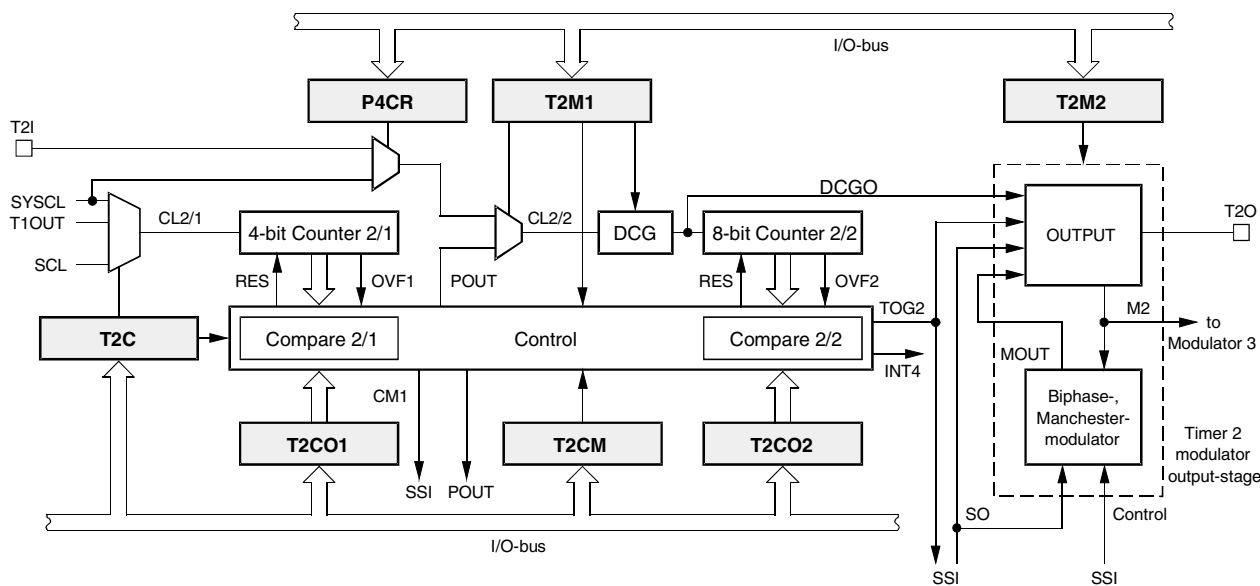
Figure 26. Timer 2
