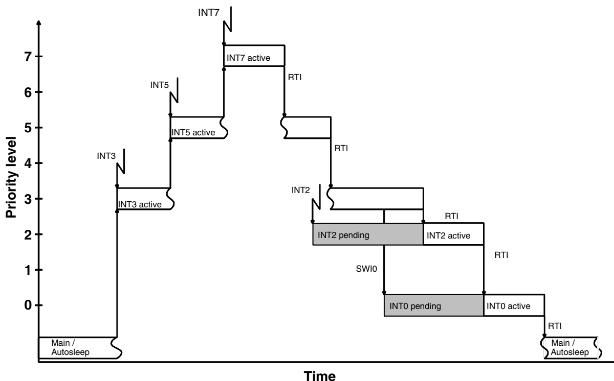
Figure 8. Interrupt Handling
