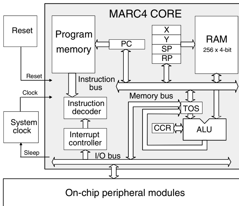
Figure 3. MARC4 Core
