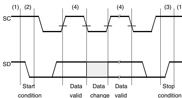
Figure 46. MCL Bus Protocol 1
