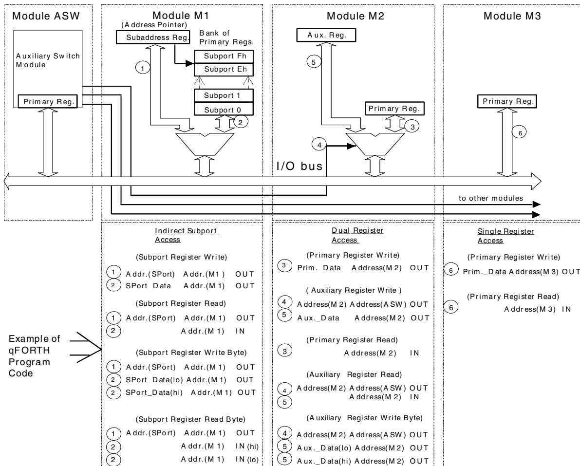
Figure 18. Example of I/O Addressing
