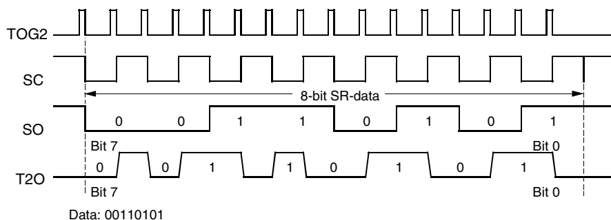
Figure 52. Manchester Modulation 1
