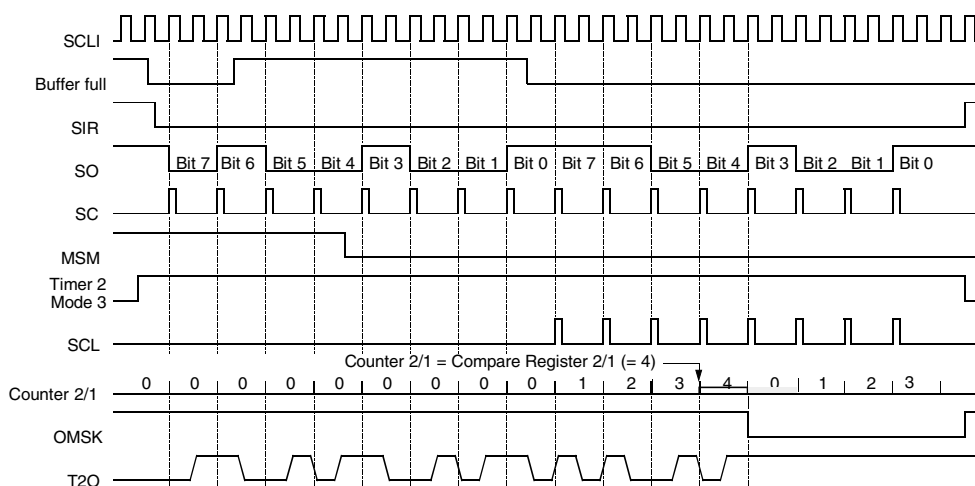
Figure 53. Manchester Modulation 2
