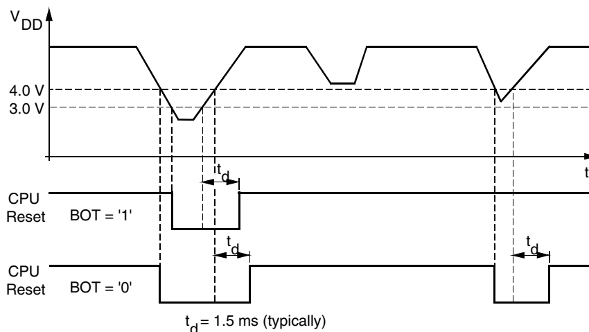
Figure 10. Brown-out Detection
