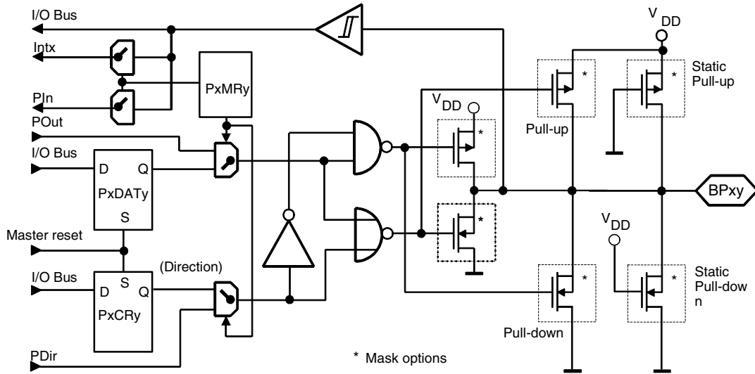
Figure 22. Bi-directional Port 4
