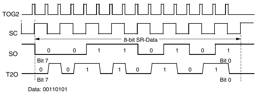
Figure 37. Manchester Modulation
