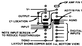
Figure 4. Suggested Layout for AD7118 and Op Amp
