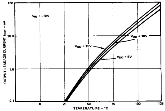
Figure 10. Output Leakage Current vs Temperature at V_{DD} = 5, 10 and 15 Volts
