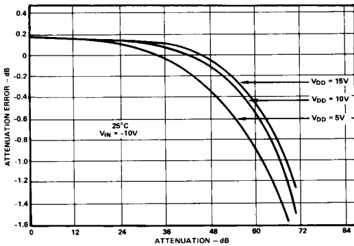
Figure 8. DC Attenuation Error vs. Attenuation & V_{DD}
