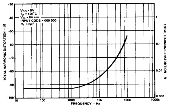
Figure 12. Distortion vs. Frequency Using AD544 Amplifier
