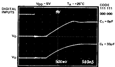
Figure 6. Response of AD7118 with AD544S
