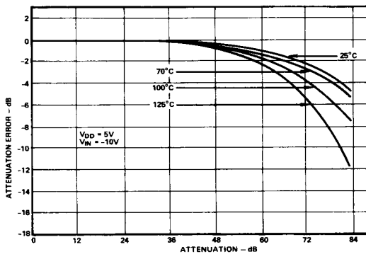
Figure 9. DC Attenuation Error vs. Attenuation & Temperature
