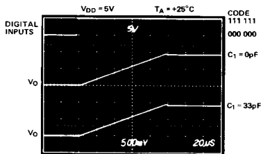
Figure 5. Response of AD7118 with AD517L
