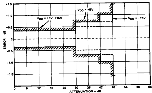
Accuracy Specification for L/C/U Grade Devices at T_A = +25^\circ C
