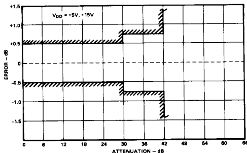
Accuracy Specification for K/B/T Grade Devices at T_A = +25^\circ C
