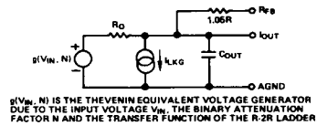
Figure 3. Equivalent Analog Output Circuit of AD7118
