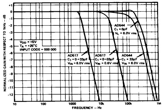
Figure 11. Frequency Response with AD544 and AD517 Amplifiers
