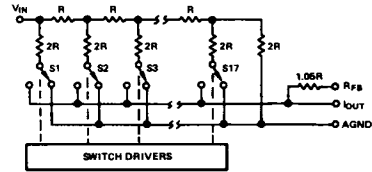
Figure 2. Simplified D/A Circuit of AD7118
