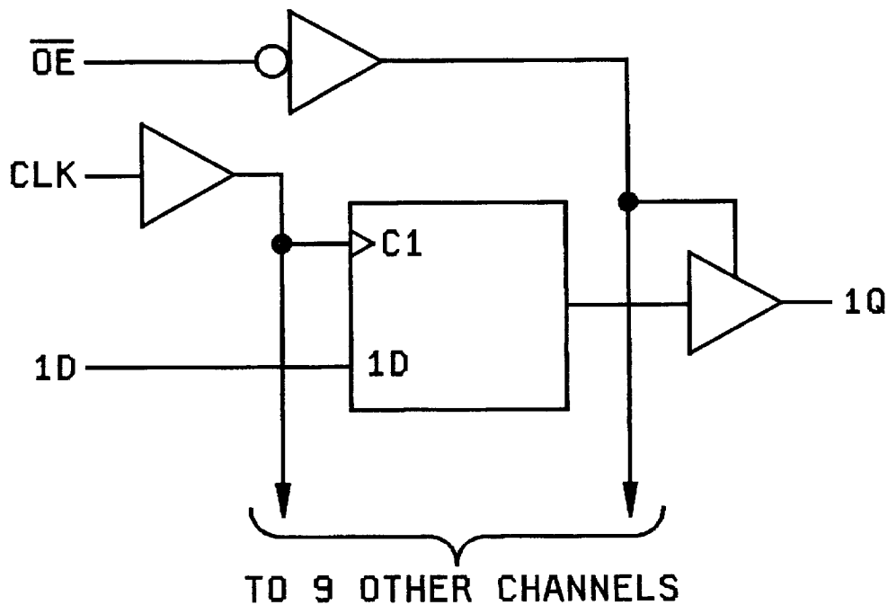
FIGURE 3. Logic diagram.
