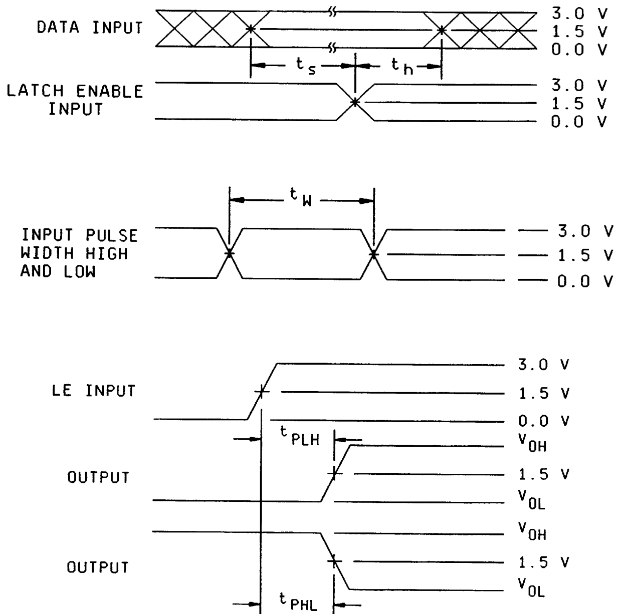
FIGURE 5. Switching waveforms and test circuit.
