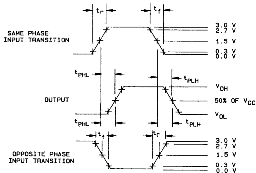
FIGURE 4. Test circuit and switching waveforms.
