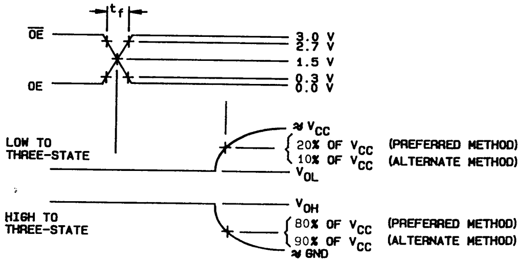
FIGURE 4. Test circuit and switching waveforms - Continued.
