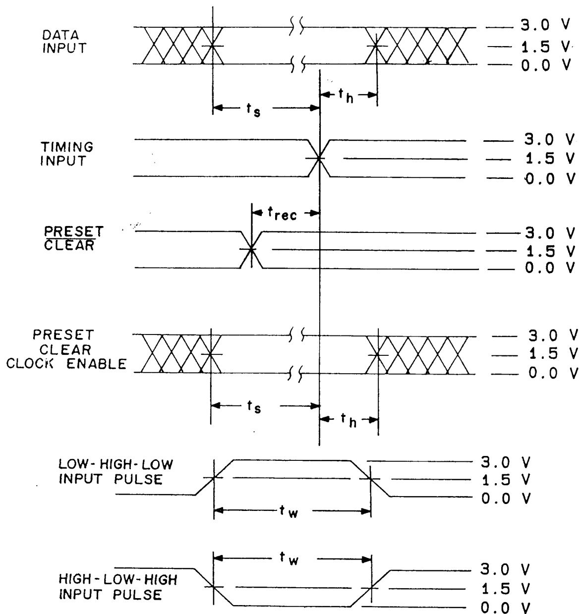
FIGURE 4. Test circuit and switching waveforms - Continued.
