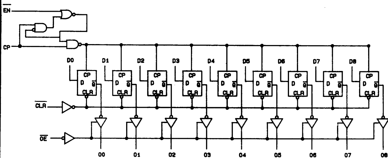
FIGURE 3. Logic diagram.
