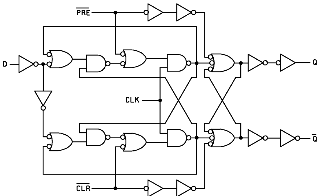
FIGURE 3. Logic diagram.
