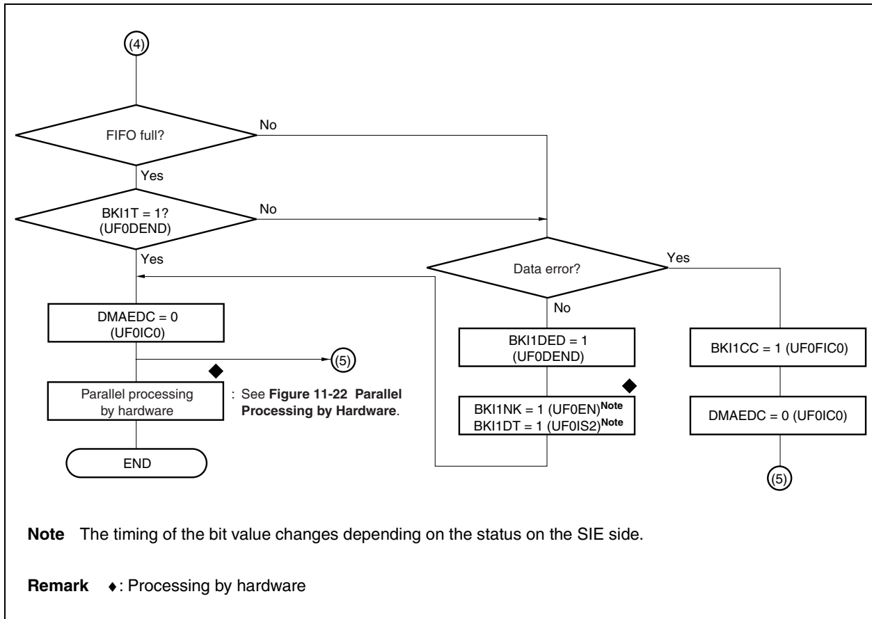
Figure 11-29. DMA Processing by Bulk Transfer (IN) (4/4)
