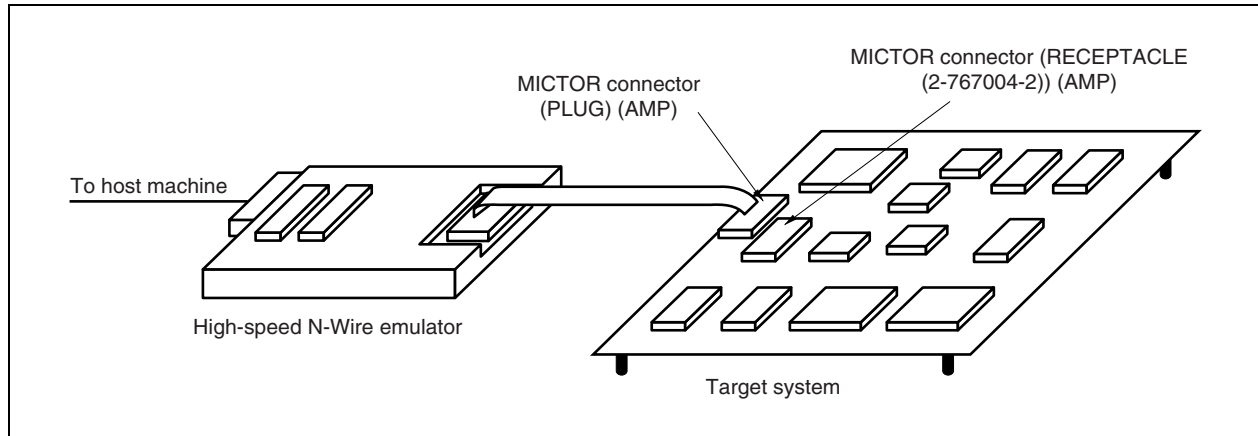
Figure 16-1. Connecting N-Wire Type IE
