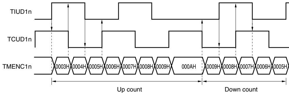
Figure 9-25. Mode 4
