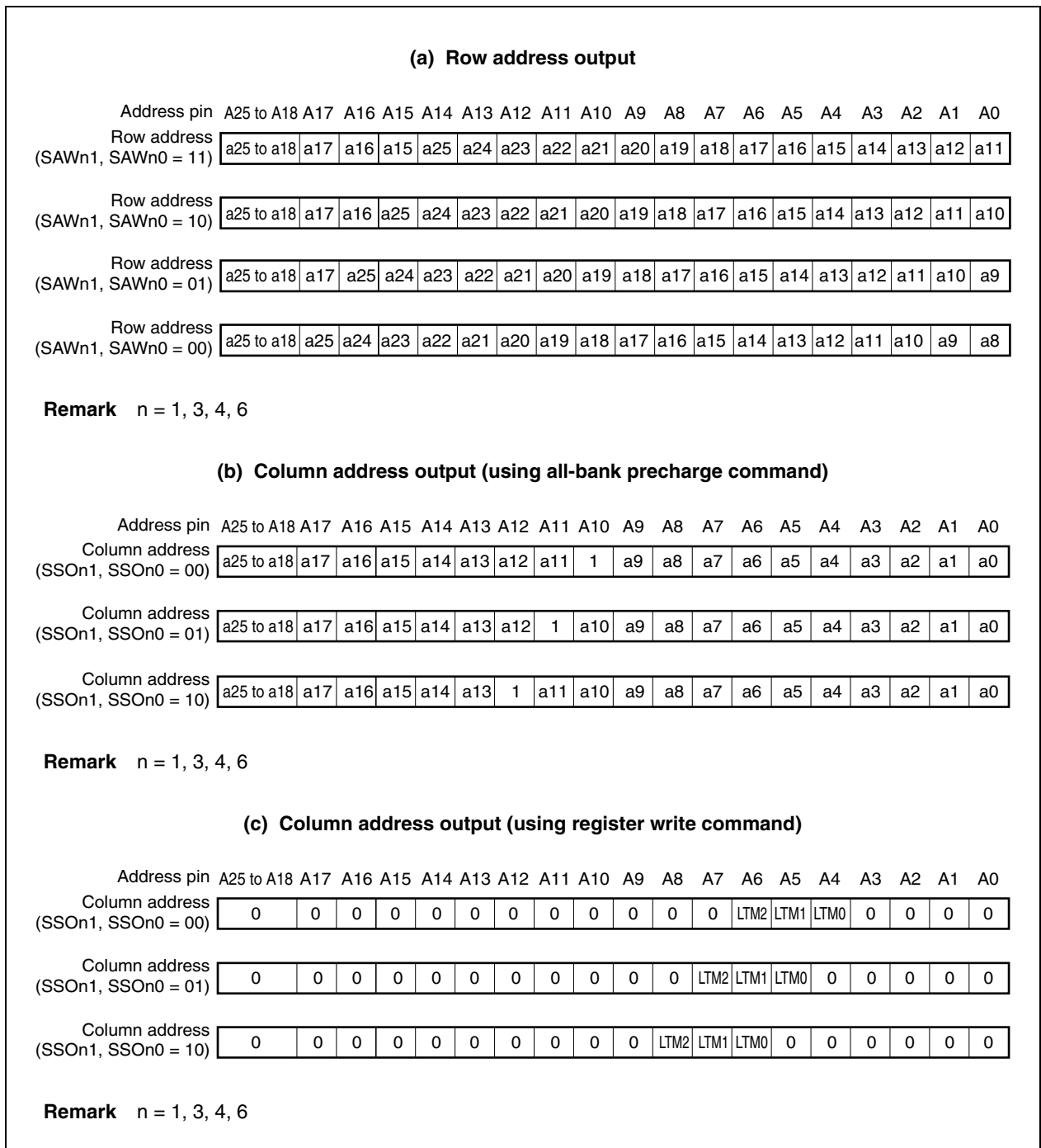
Figure 5-7. Row Address/Column Address Output (1/2)
