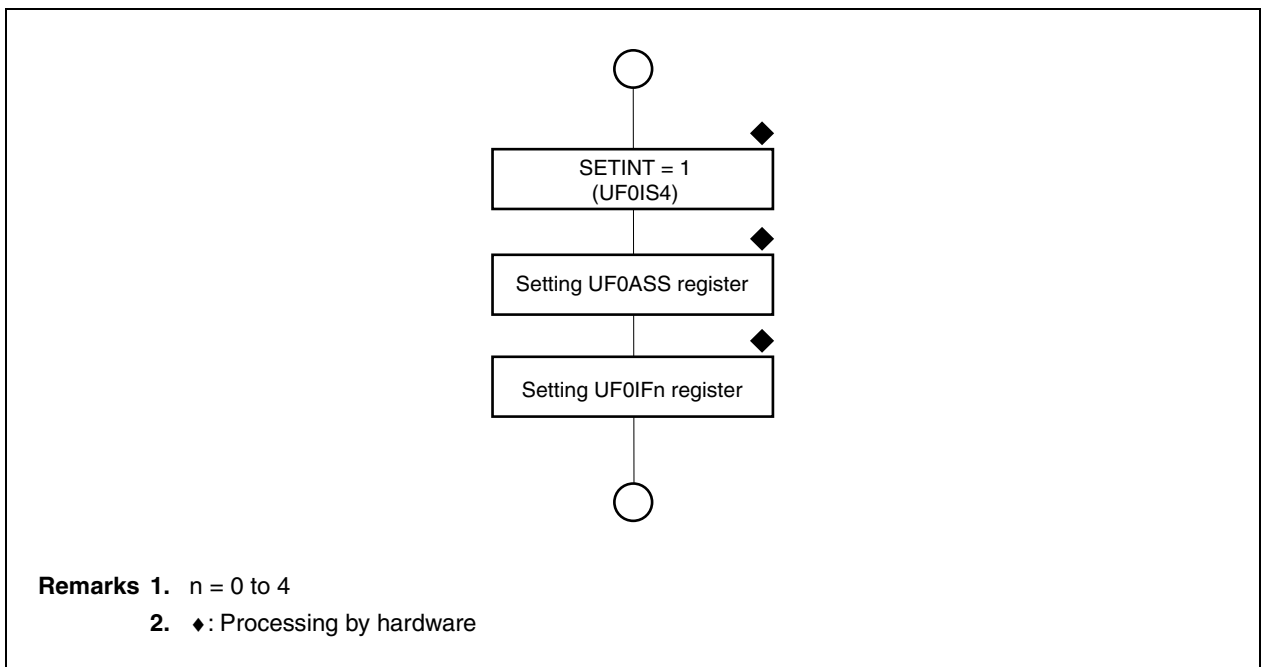
Figure 11-19. SET_INTERFACE Processing
