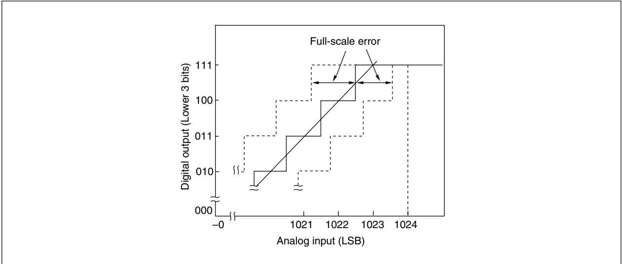
Figure 12-18. Full-Scale Error
