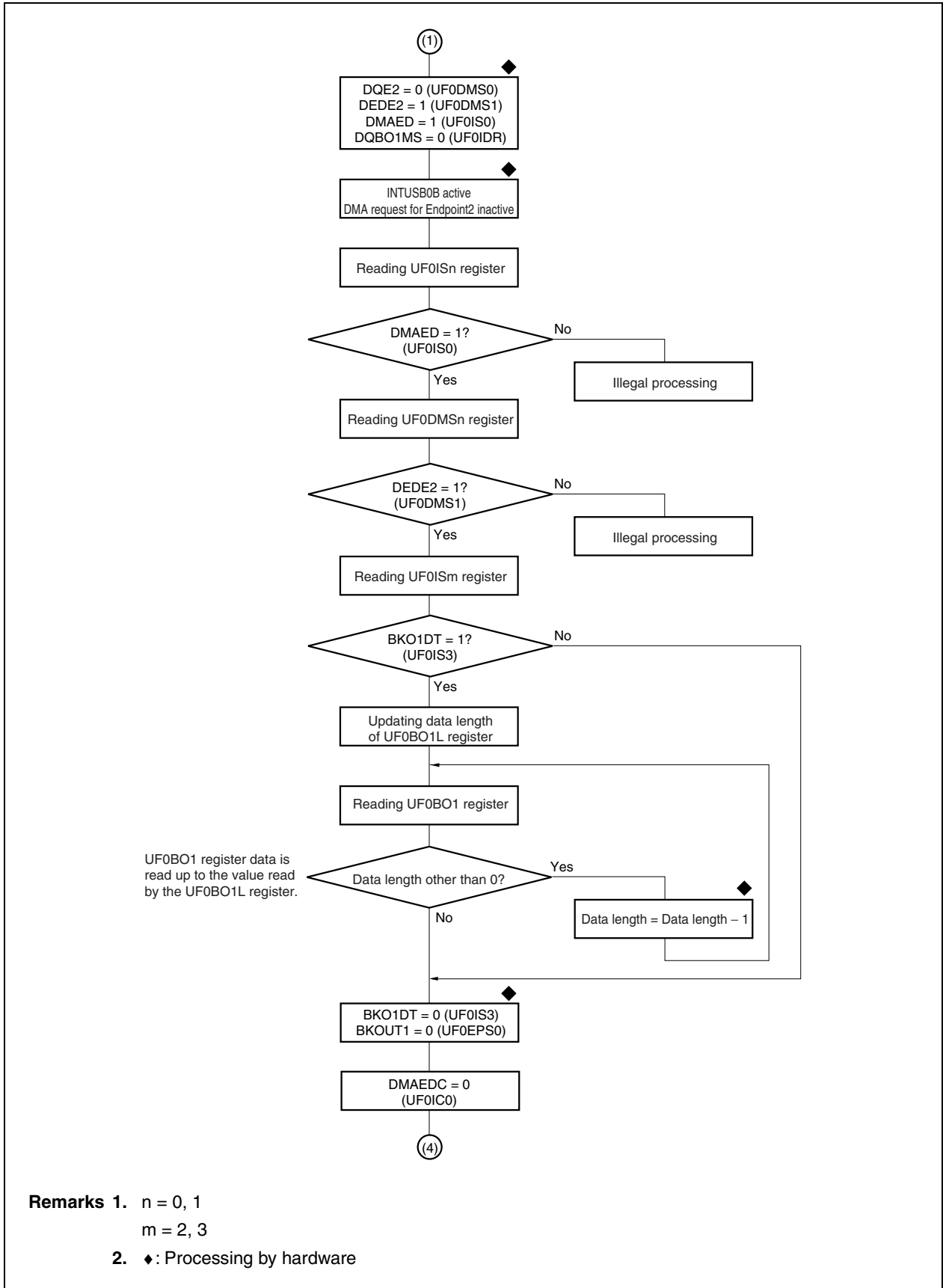
Figure 11-28. DMA Processing by Bulk Transfer (OUT) (3/3)
