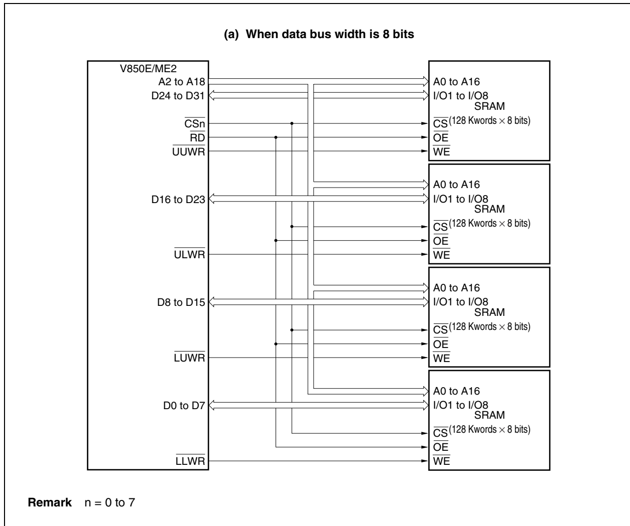
Figure 5-1. Examples of Connection to SRAM (1/2)
