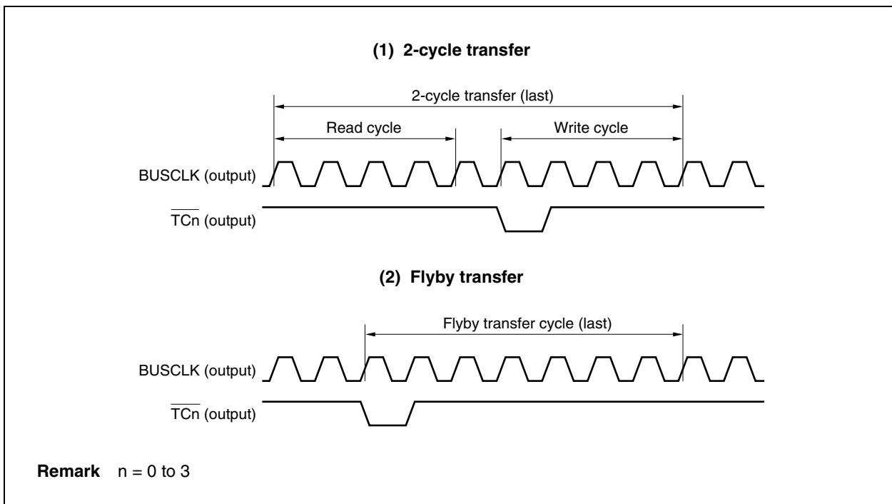
Figure 6-27. Terminal Count Signal ( \overline{TCn} ) Timing Example (2)
