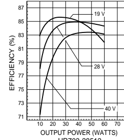
HR703-28512 EFFICIENCY VS. LINE & LOAD FIGURE 8
