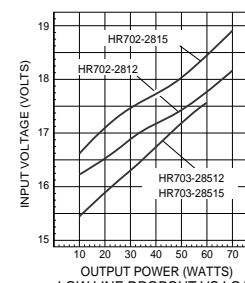
HR702-2815 HR702-2812 HR703-28512 HR703-28515 LOW LINE DROPOUT VS LOAD (50mV DROP) FIGURE 11
