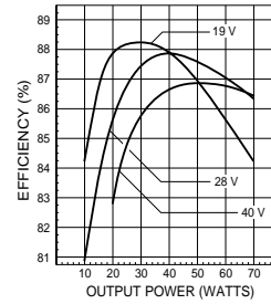
HR701-2815 EFFICIENCY VS. LINE & LOAD FIGURE 5
