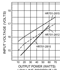
HR701-2815 LOW LINE DROPOUT VS LOAD (50mV DROP) FIGURE 10
