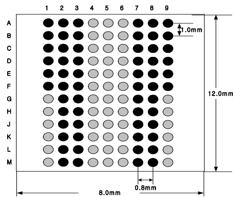
BGA Package Ball Pattern Top View
