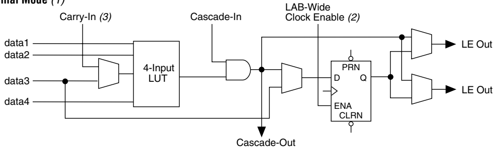
Figure 8. APEX 20KC LE Operating Modes
