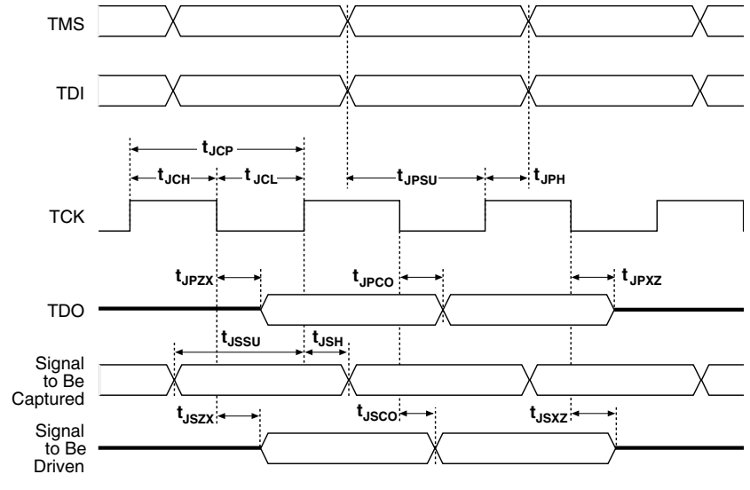
Figure 30. APEX 20KC JTAG Waveforms
