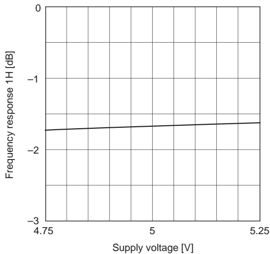
Frequency response (1H) vs. Supply voltage
