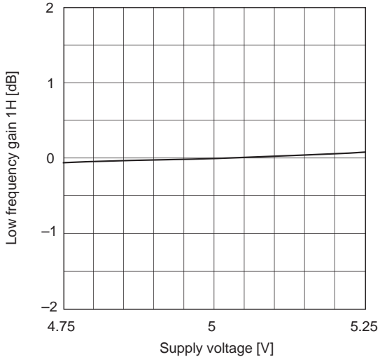
Low frequency gain (1H) vs. Supply voltage
