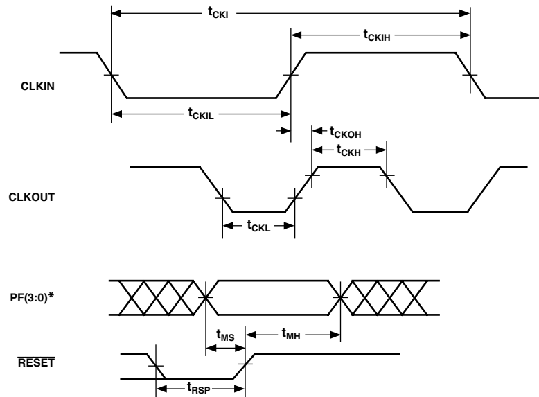
Figure 21. Clock Signals
