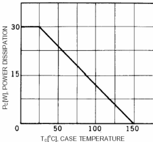
Fig.7 Power Derating
