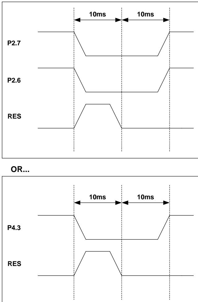
FIGURE 4: VRS51C1100 ALTERNATE ISP BOOT PROGRAM ACCESS
