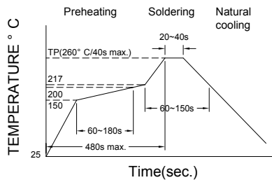
Figure 1. Re-flow Soldering
