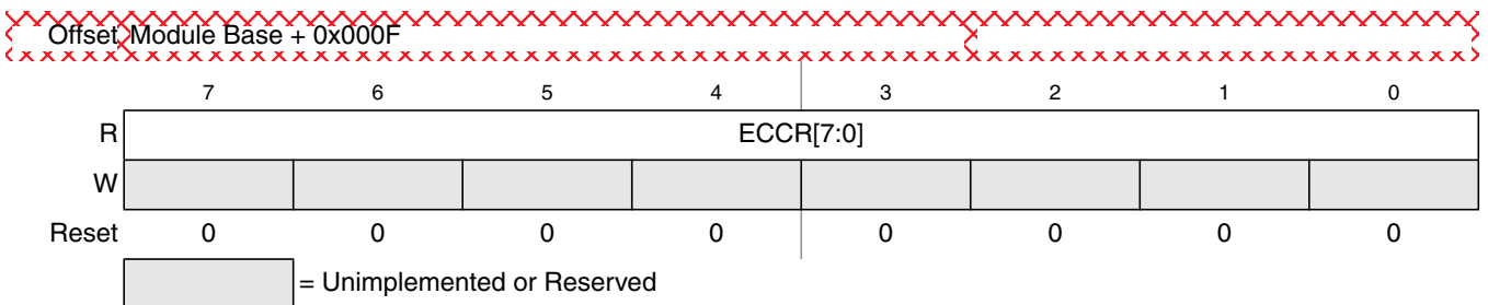
Figure 26-21. Flash ECC Error Results Low Register (FECCRLO)
