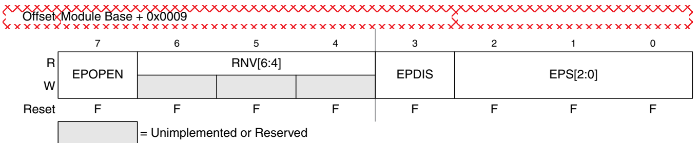
Figure 27-15. EEE Protection Register (EPROT)
