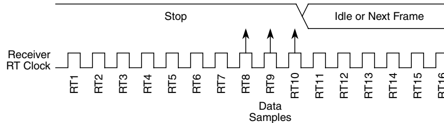
Figure 20-29. Fast Data
