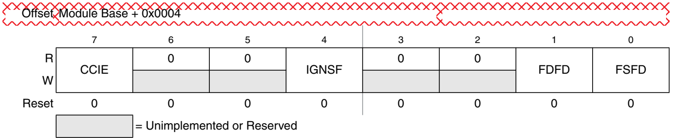
Figure 26-9. Flash Configuration Register (FCNFG)
