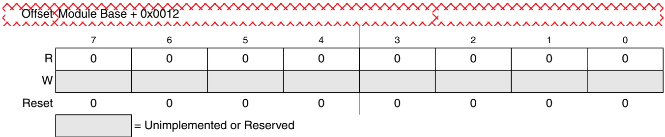
Figure 29-24. Flash Reserved 1 Register (FRSV 1 )
