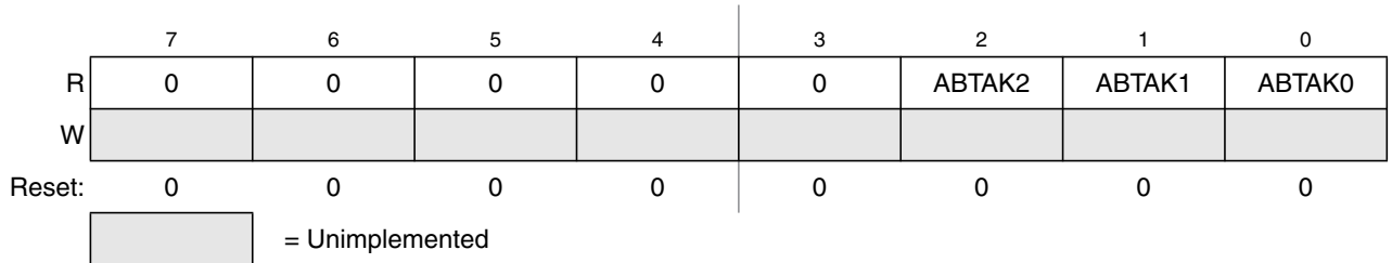
Figure 16-13. MSCAN Transmitter Message Abort Acknowledge Register (CANTAACK)
