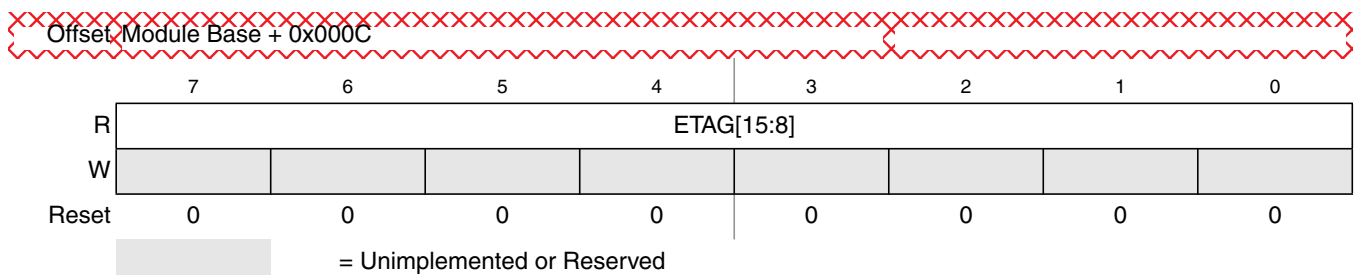
Figure 26-18. EEE Tag Counter High Register (ETAGHI)
