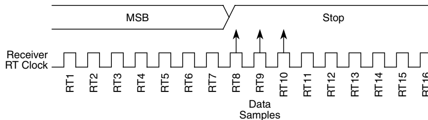
Figure 20-28. Slow Data
