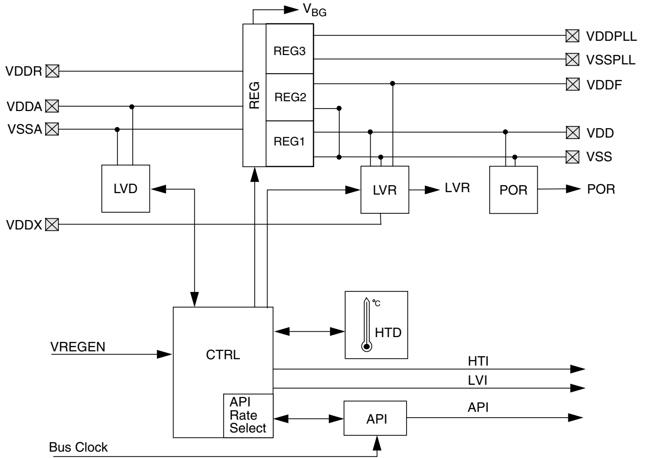
Figure 23-1. VREG_3V3 Block Diagram
