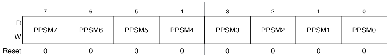
Figure 2-40. Port M Polarity Select Register (PPSM)
