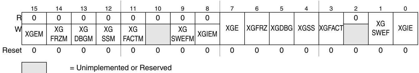
Figure 10-3. XGATE Control Register (XGMCTL)
