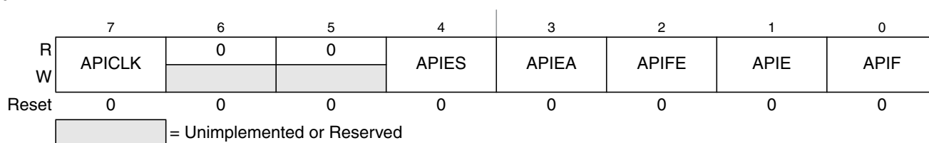
Figure 23-3. Autonomous Periodical Interrupt Control Register (VREGAPICL)
