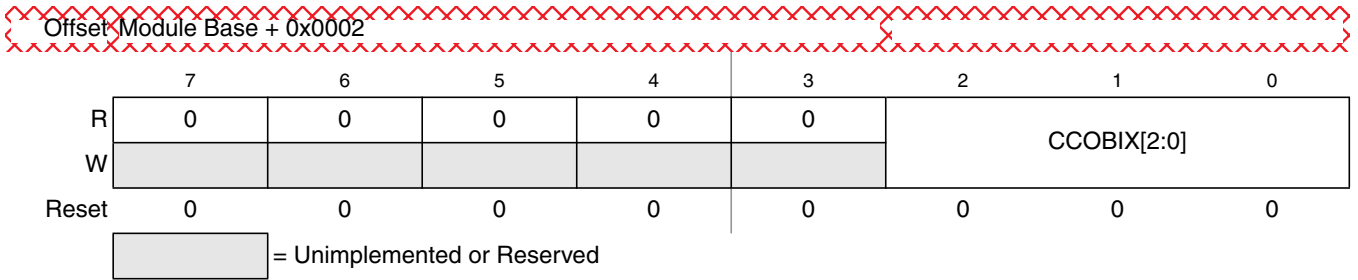
Figure 29-7. FCCOB Index Register (FCCOBIX)
