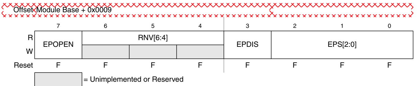
Figure 26-15. EEE Protection Register (EPROT)
