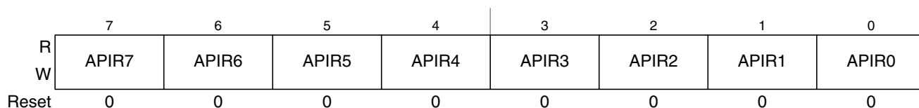
Figure 23-6. Autonomous Periodical Interrupt Rate Low Register (VREGAPIRL)
