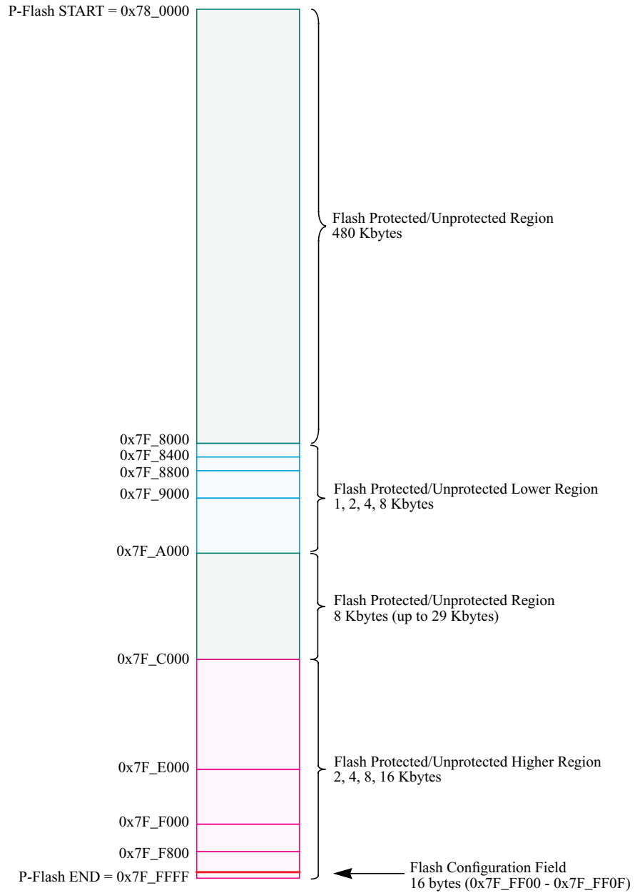
Figure 27-2. P-Flash Memory Map
