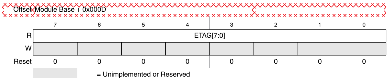
Figure 27-19. EEE Tag Counter Low Register (ETAGLO)
