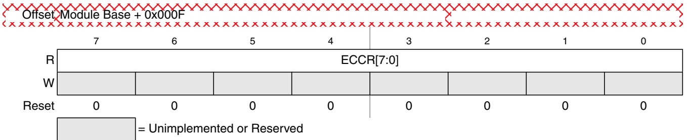
Figure 29-21. Flash ECC Error Results Low Register (FECCRLO)
