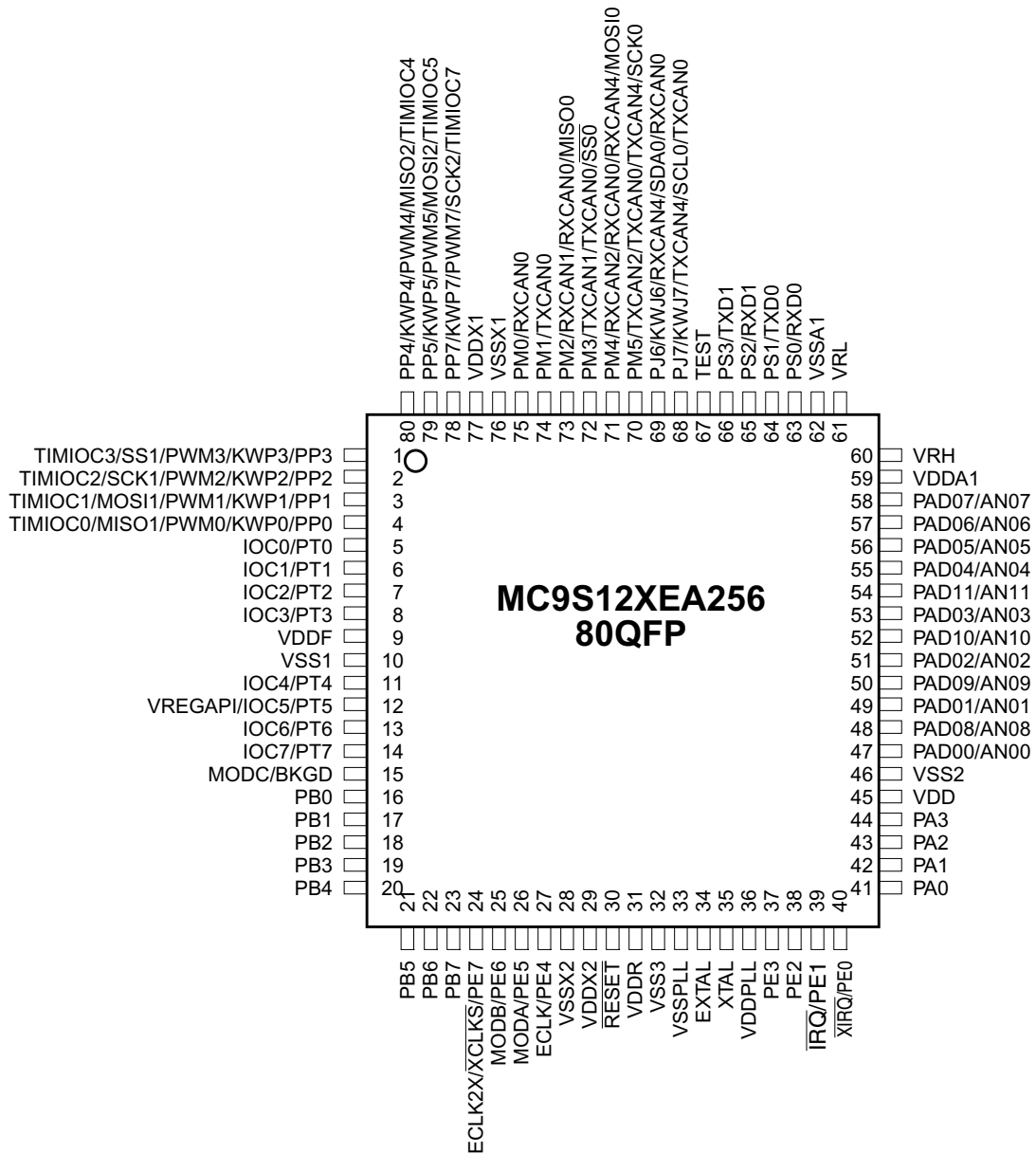
Figure 1-8. MC9S12XEA256 80-pin QFP Package Pin Assignment
