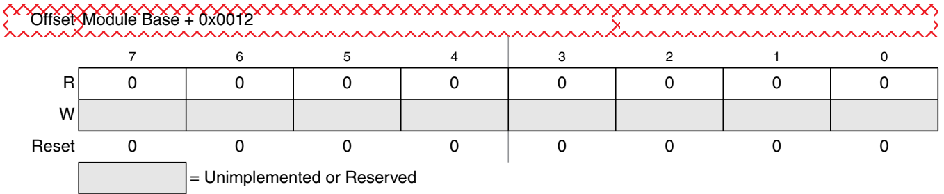
Figure 26-24. Flash Reserved 1 Register (FRSV 1 )
