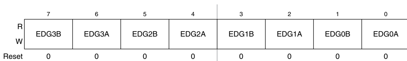
Figure 22-17. Timer Control Register 4 (TCTL4)
