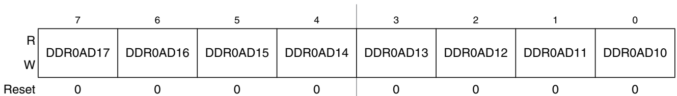
Figure 2-77. Port AD1 Data Direction Register 0 (DDR0AD1)
