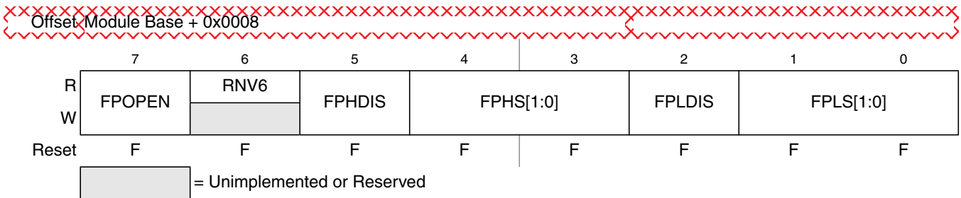
Figure 26-13. Flash Protection Register (FPROT)
