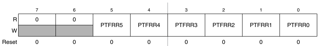
Figure 2-106. Port F Routing Register (PTFRR)
