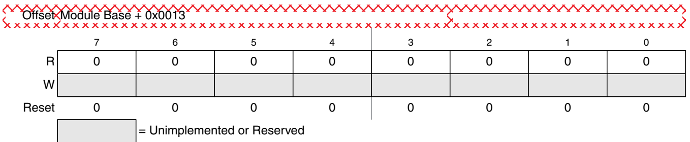
Figure 27-25. Flash Reserved2 Register (FRSV2)
