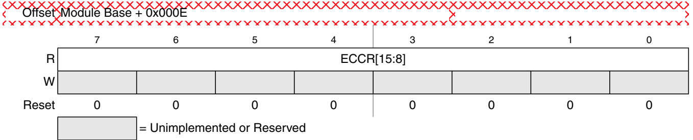
Figure 27-20. Flash ECC Error Results High Register (FECCRHI)
