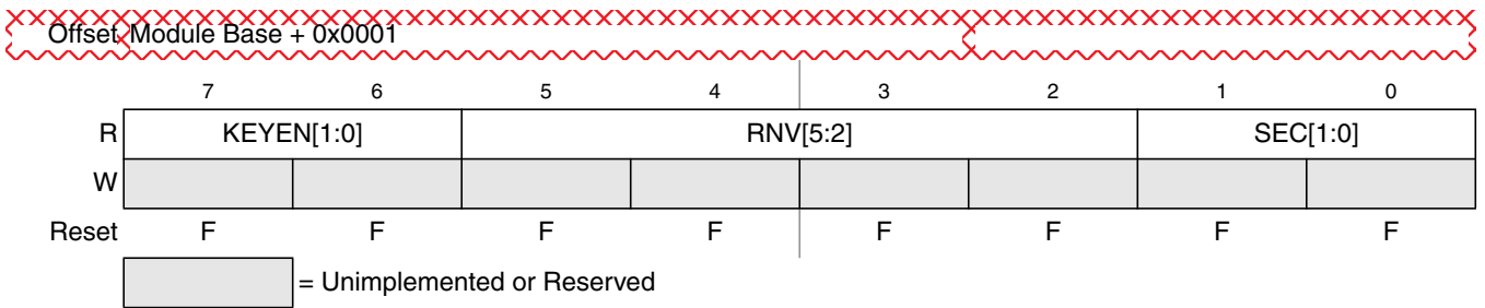
Figure 26-6. Flash Security Register (FSEC)
