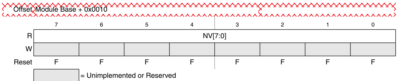
Figure 27-22. Flash Option Register (FOPT)
