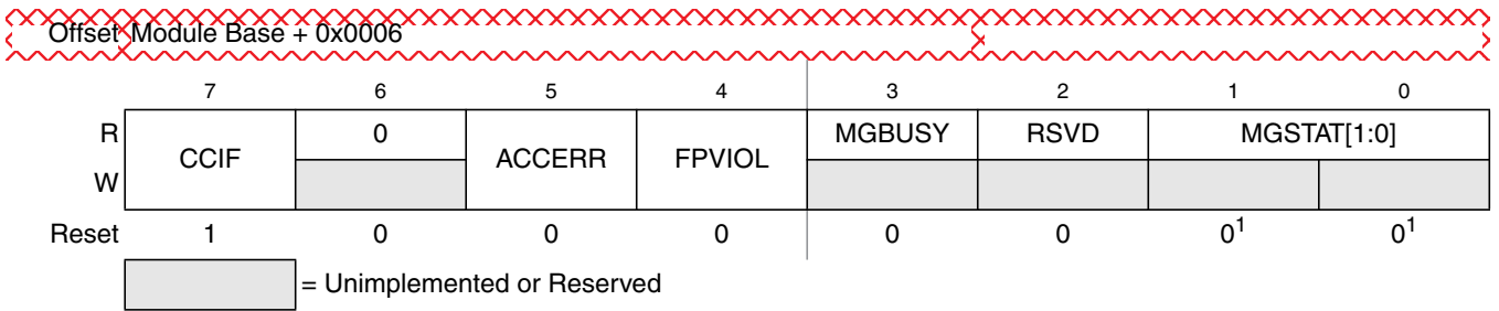
Figure 27-11. Flash Status Register (FSTAT)
