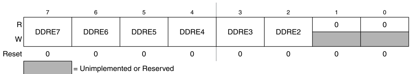
Figure 2-10. Port E Data Direction Register (DDRE)
