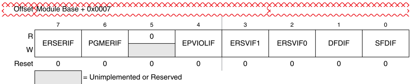
Figure 27-12. Flash Error Status Register (FERSTAT)
