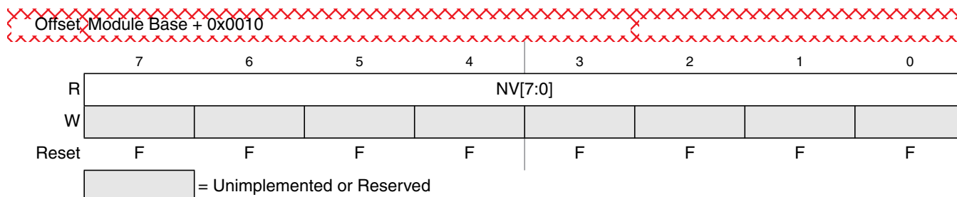
Figure 29-22. Flash Option Register (FOPT)
