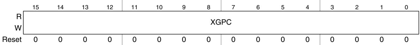
Figure 10-14. XGATE Program Counter Register (XGPC)
