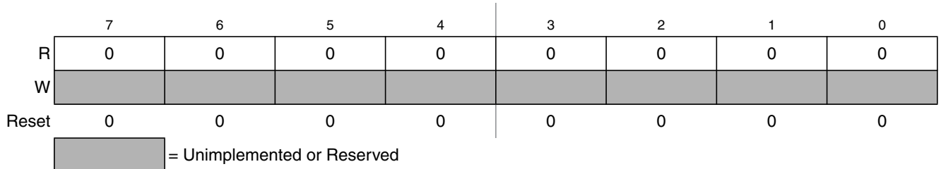
Figure 2-14. PIM Reserved Register
