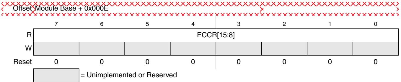
Figure 29-20. Flash ECC Error Results High Register (FECCRHI)
