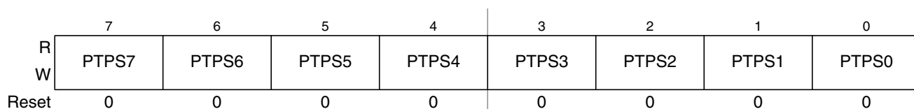
Figure 22-29. Precision Timer Prescaler Select Register (PTPSR)
