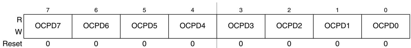
Figure 22-28. Output Compare Pin Disconnect Register (OCPD)
