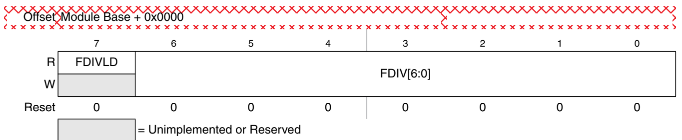
Figure 27-5. Flash Clock Divider Register (FCLKDIV)
