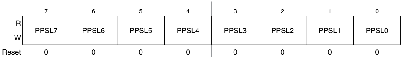
Figure 2-96. Port L Polarity Select Register (PPSL)
