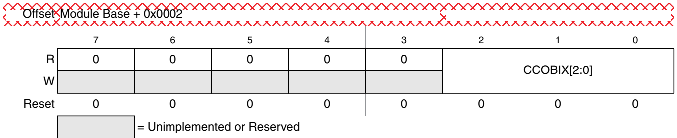
Figure 26-7. FCCOB Index Register (FCCOBIX)
