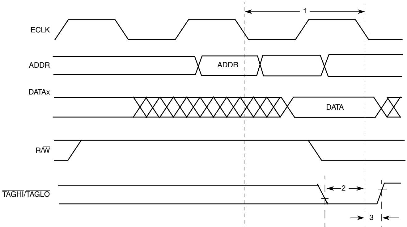
Figure A-18. External Trigger Timing
