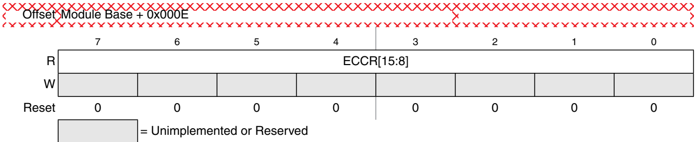
Figure 26-20. Flash ECC Error Results High Register (FECCRHI)
