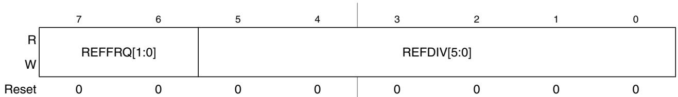
Figure 11-4. S12XECRG Reference Divider Register (REFDV)
