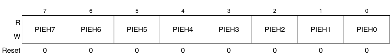
Figure 2-57. Port H Interrupt Enable Register (PIEH)
