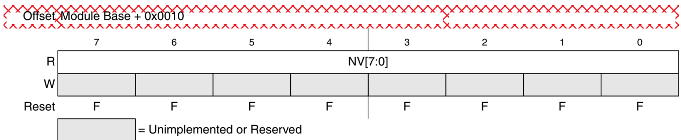
Figure 26-22. Flash Option Register (FOPT)
