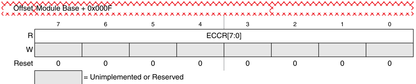
Figure 27-21. Flash ECC Error Results Low Register (FECCRLO)
