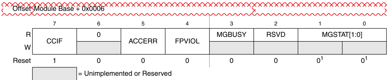
Figure 26-11. Flash Status Register (FSTAT)
