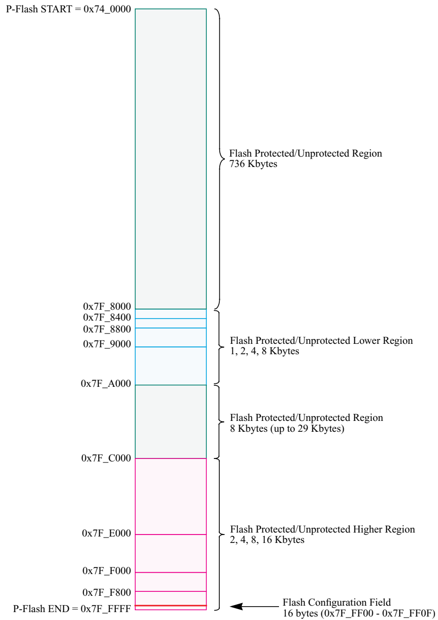
Figure 28-2. P-Flash Memory Map
