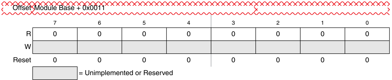
Figure 26-23. Flash Reserved 0 Register (FRSV 0 )
