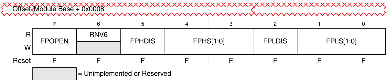
Figure 27-13. Flash Protection Register (FPROT)
