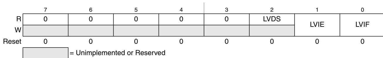
Figure 23-2. Control Register (VREGCTRL)
