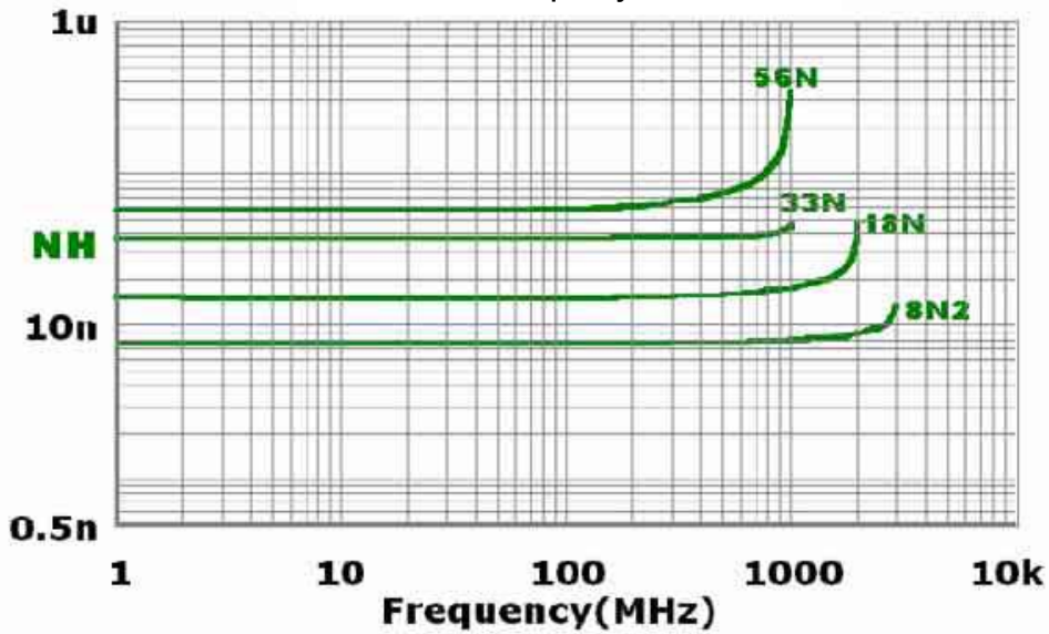
Inductance vs. Frequency Characteristics
