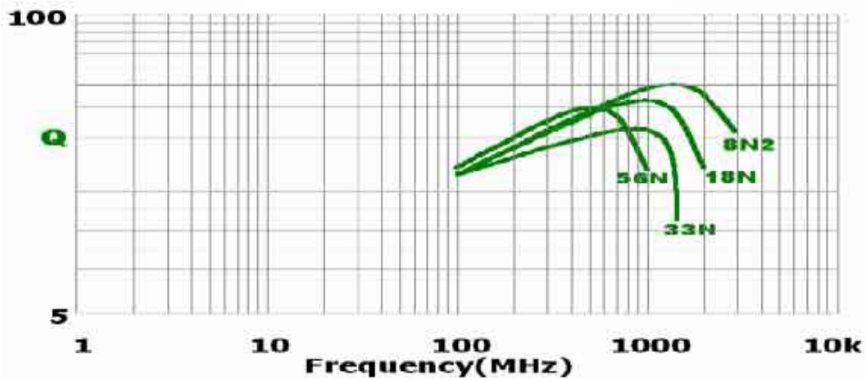
Q vs. Frequency Characteristics
