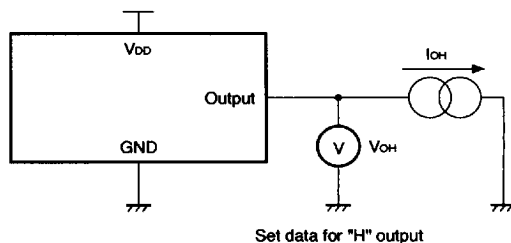
Fig. 2 "H" output voltage measurement circuit
