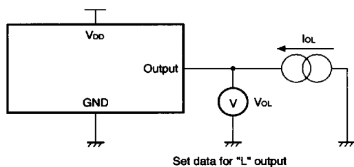
Fig. 1 "L" output voltage measurement circuit
