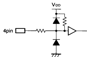
Input with pullup resistor
