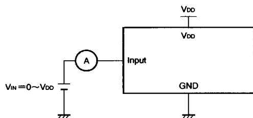
Fig. 3 Input leakage current, input voltage measurement circuit
