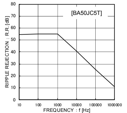
Fig.6 Ripple Rejection
