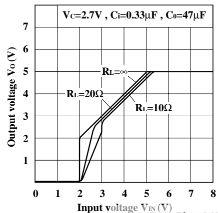
Fig.8 Output Voltage vs. Input Voltage (PQ05TZ51)
