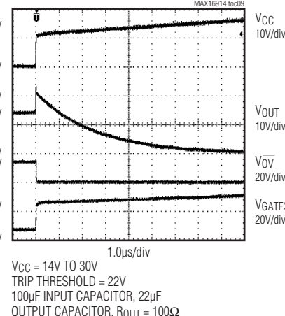
OVERVOLTAGE SWITCH-OFF RESPONSE (MAX16914)
