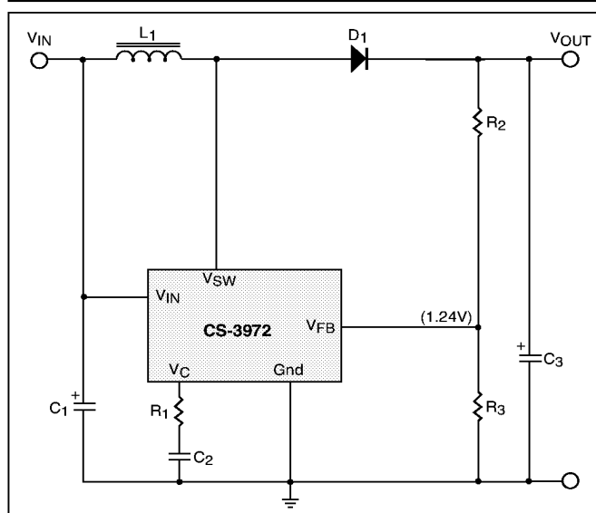
Figure 1: Boost Regulator
