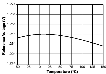
Reference Voltage vs. Temperature
