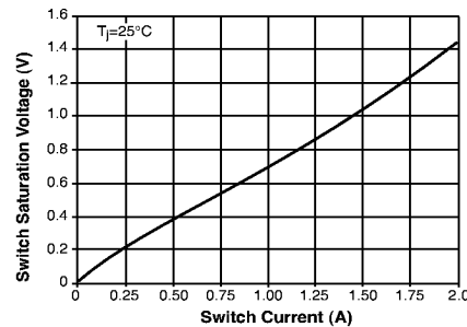
Switch Saturation Voltage
