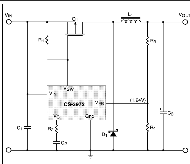
Figure 2: Buck Regulator with the External Switch
