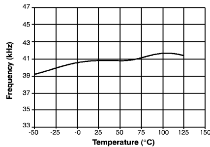
Switching Frequency vs. Temperature
