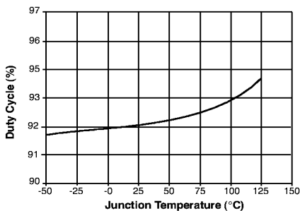
Maximum Duty Cycle
