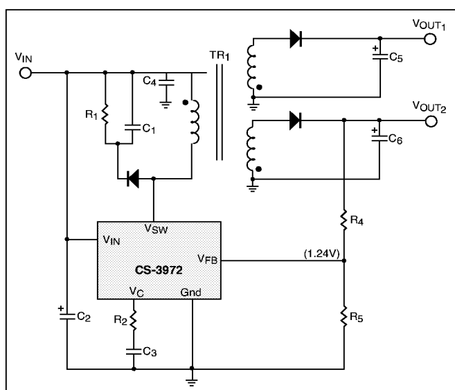
Figure 3:: Flyback Multiple Output Regulator
