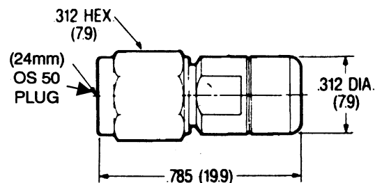
OS-50 (2.4 mm) Figure 1
