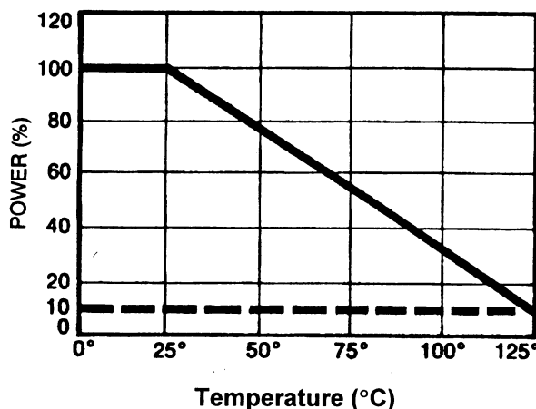
Typical Power Derating
