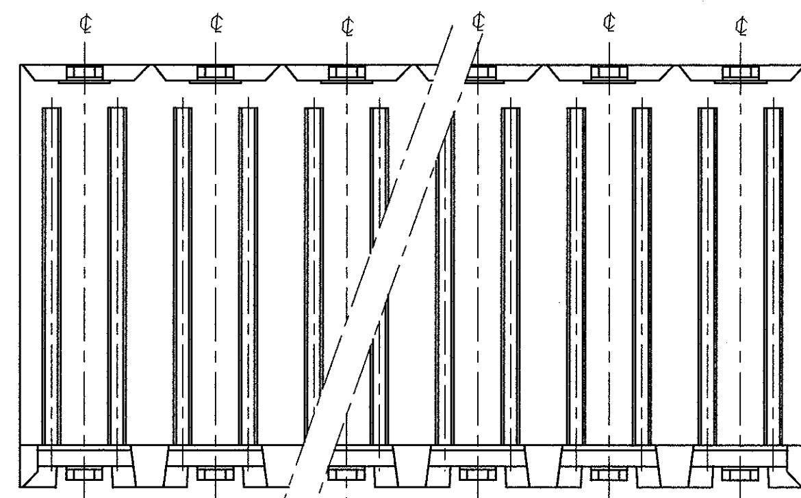
BOTTOM VIEW
