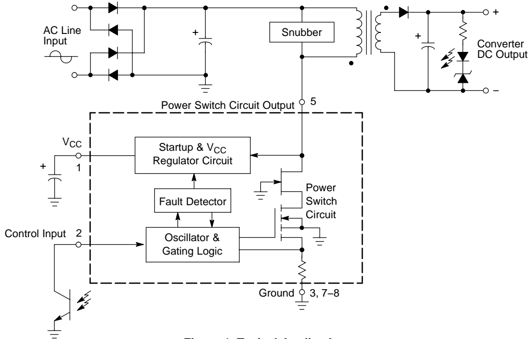
Figure 1. Typical Application
