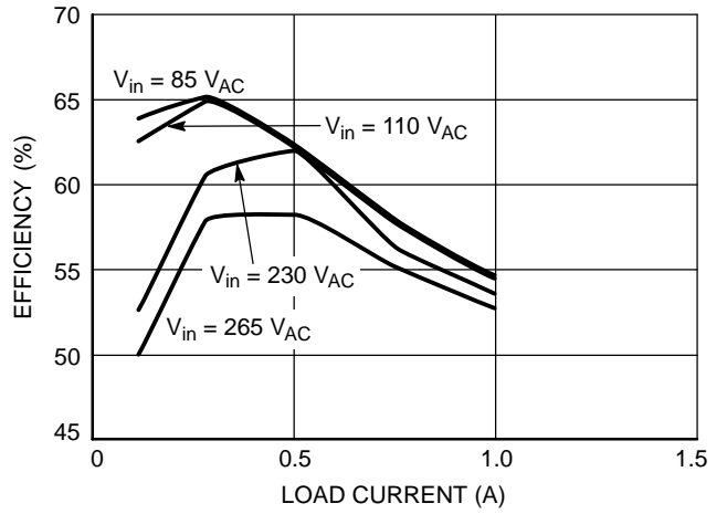
Figure 37. Charger Efficiency
