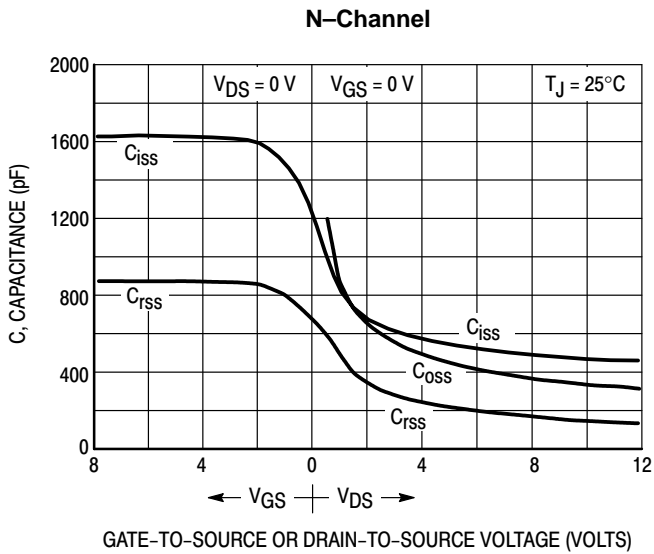
Figure 7. Capacitance Variation
