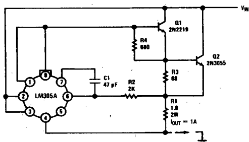
Current Regulator
