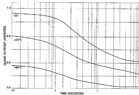
TYPICAL TRIP CURRENT VS TIME FIGURE 7 (See Note 5)
