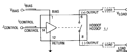
(E) 3 Terminal Input without Status
