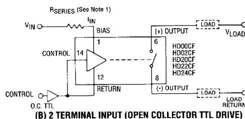
(B) 2 Terminal Input (Open Collector TTL Drive)
