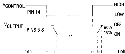
OUTPUT TURN-ON AND TURN-OFF TIMING FIGURE 5
