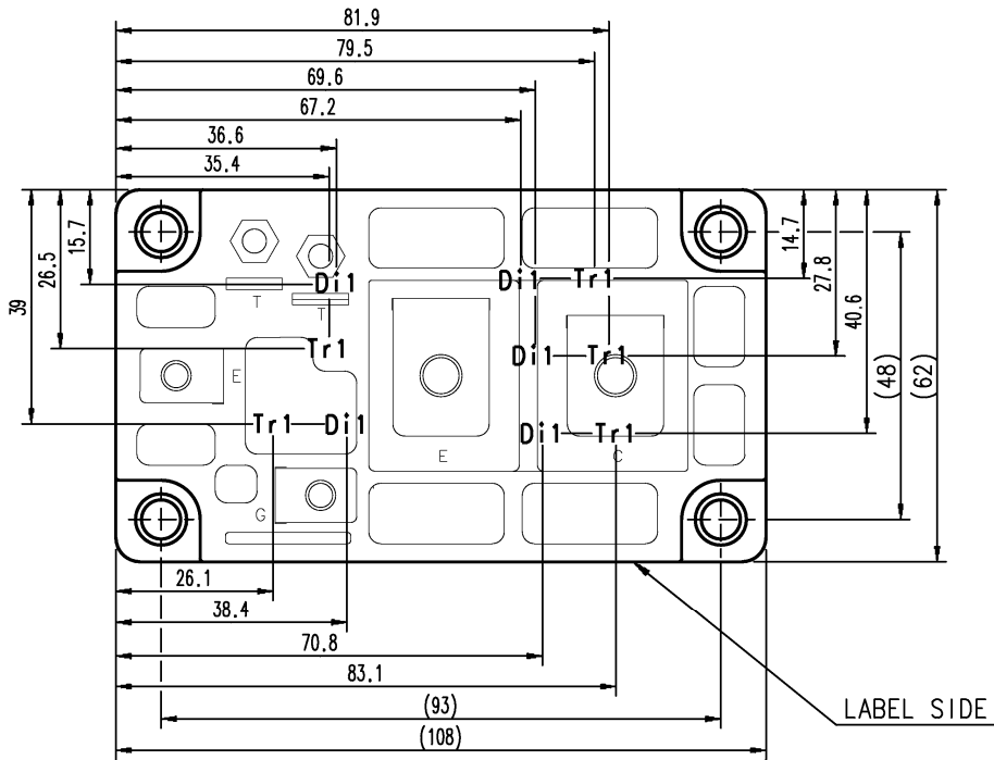
Tr1: IGBT, Di1: FWDi. Each mark points the center position of each chip.
