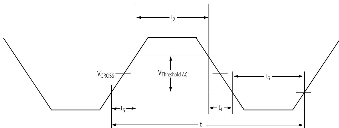
Figure 8. SYSCLK Waveform
