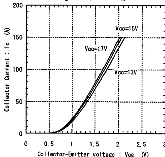
Collector current vs. Collector-Emmitter voltage T_j=25^\circ\text{C} (Terminal)
