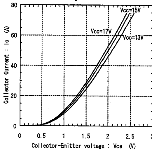
Collector current vs. Collector-Emitter voltage T_J=125^{\circ}\text{C}
