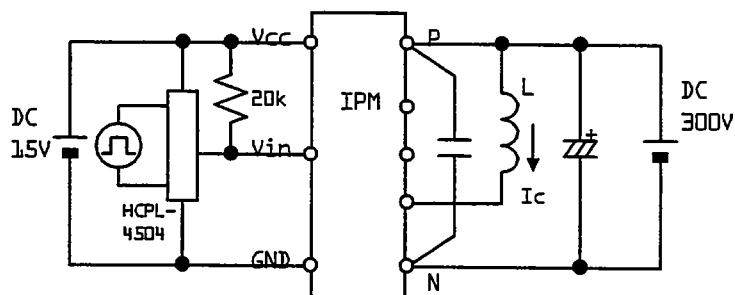
Figure 6. Switching Characteristics Test Circuit
