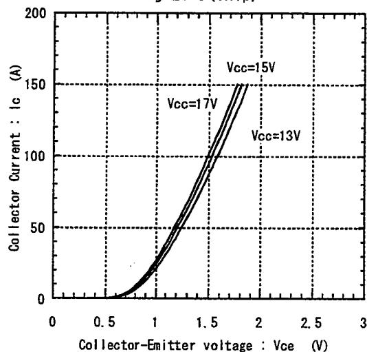
Collector current vs. Collector-Emmitter voltage T_j=25^\circ\text{C} (Chip)
