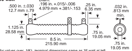
Fixed/Adjustable 300 watt*
