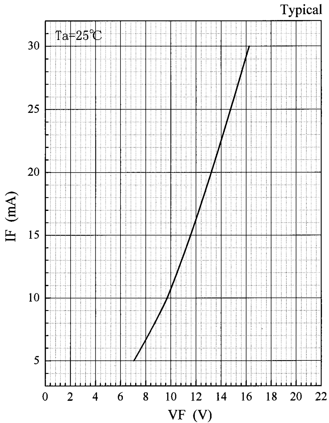
Fig.1 Forward characteristic[VF-IF]
