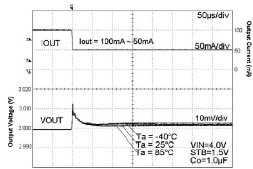
Fig. 139 Load Response
