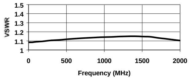
VSWR RFout 8 dB Bit & Max. Attenuation
