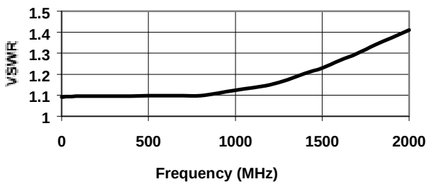
VSWR RFin 0.5, 1, 2, 4, 8 dB Bits & Max. Attenuation
