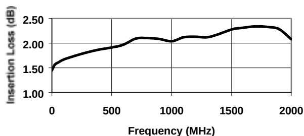
Insertion loss
