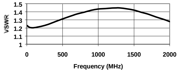
VSWR RFout 0.5, 1, 2, & 4 dB Bits
