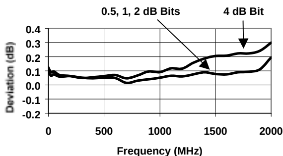
Attenuation Accuracy
