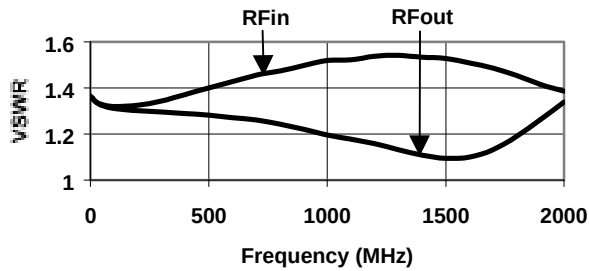
VSWR @ Insertion Loss
