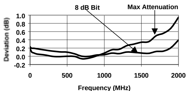
Attenuation Accuracy
