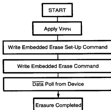
Figure 5. Embedded Erase Algorithm
