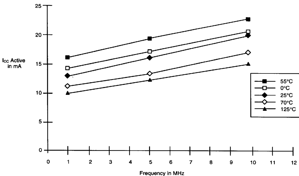
Figure 9. Am28F010A – Average I_{cc} Active vs. Frequency V_{cc} = 5.5 V, Addressing Pattern = Minmax Data Pattern = Checkerboard
