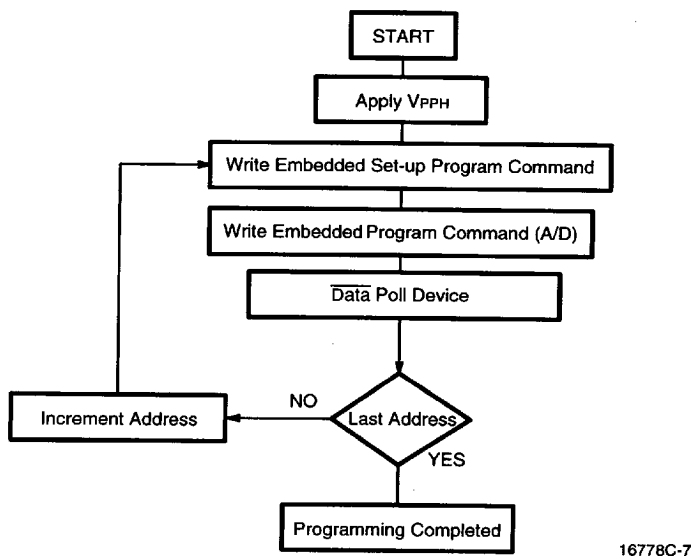
Figure 6. Embedded Program Algorithm
