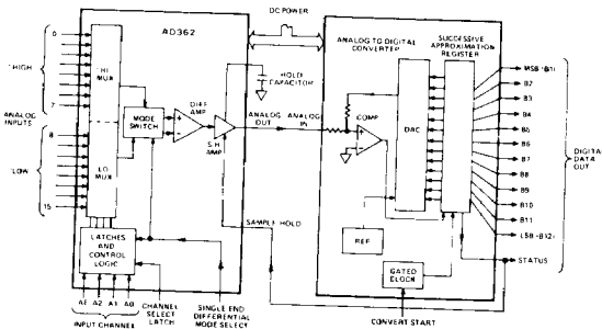
Figure 1. AD362 with ADC as a Complete Data Acquisition System
