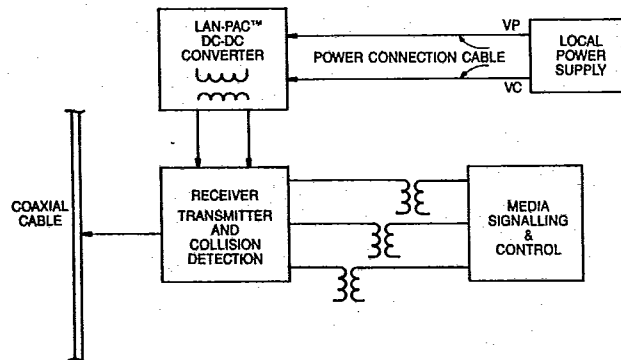
BLOCK DIAGRAM LOCAL AREA NETWORK (LAN)
