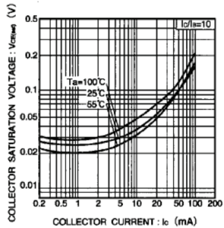
Fig.8 Collector-emitter saturation voltage vs. collector current ( II )
