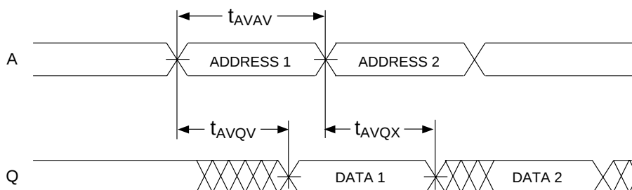
FIG. 4 READ CYCLE 1 - \overline{W} HIGH, \overline{G} , \overline{E} LOW
