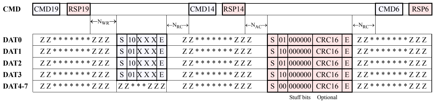
Figure 6-21: 4 bit System Bus Testing Procedure
