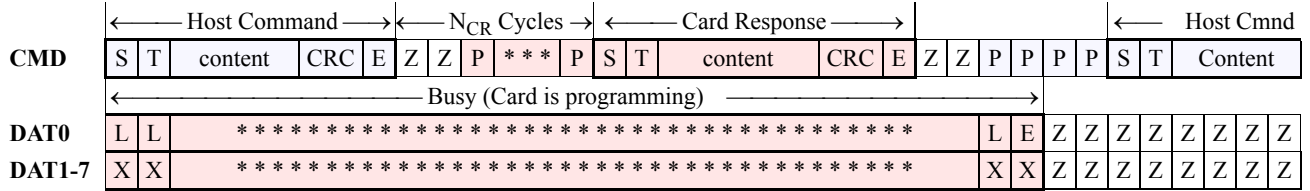
Figure 6-19 : Stop Transmission After Last Data Block. Card Is Busy Programming.
