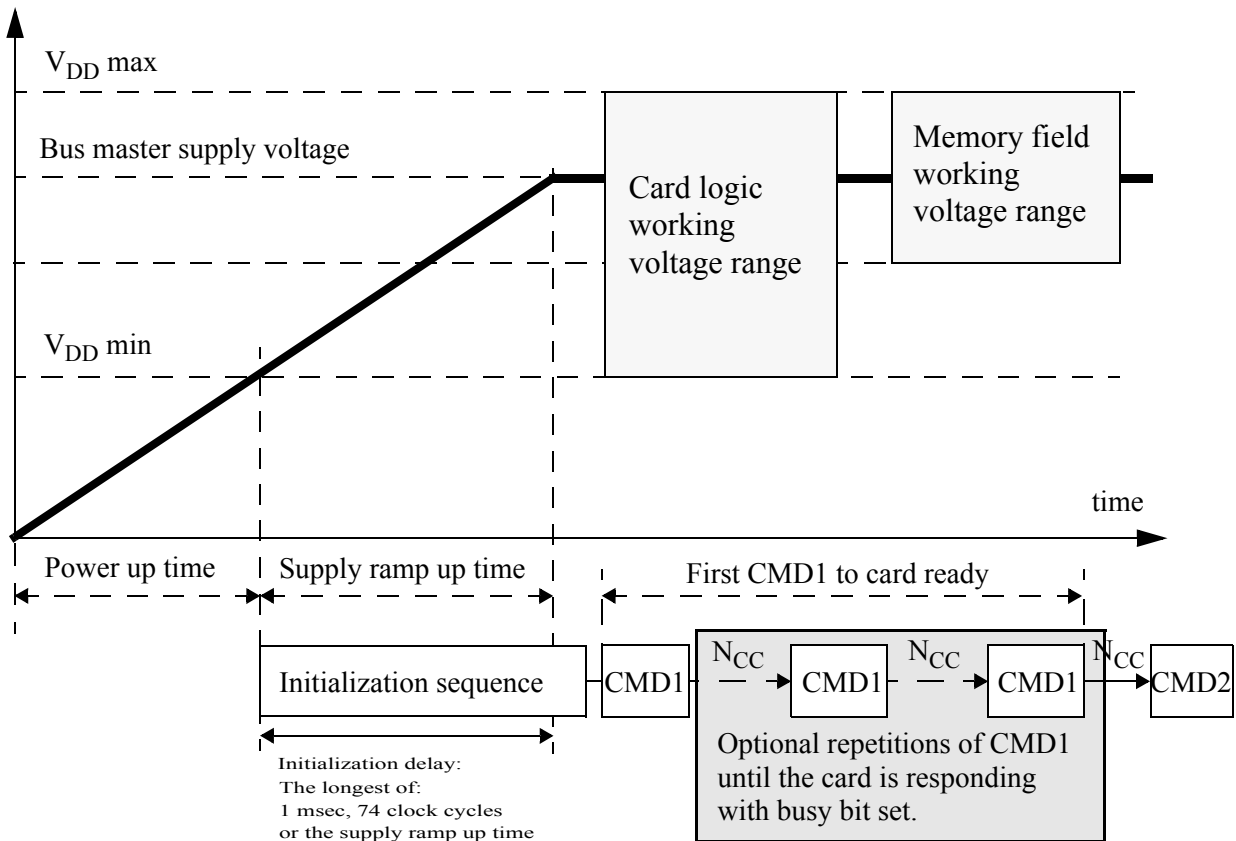
Figure 5-3 : Power-up Diagram
