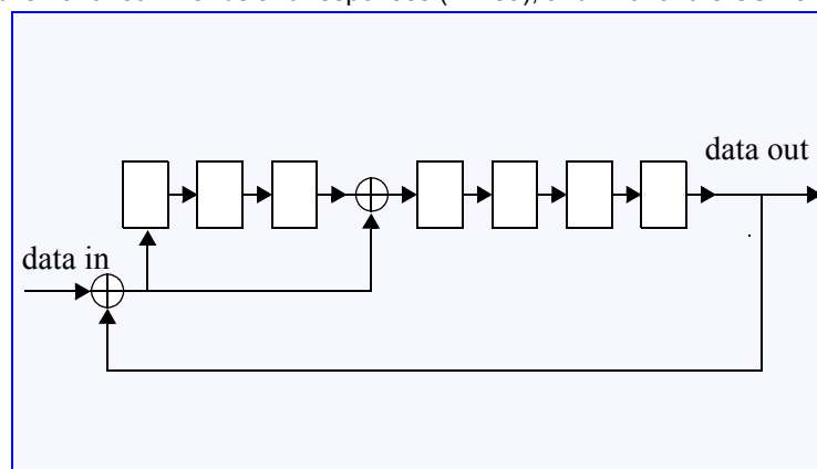
Figure 6-3 : CRC7 Generator/Checker
