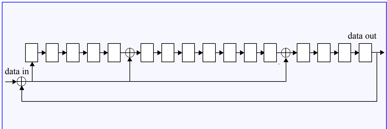
Figure 6-4 : CRC16 Generator/Checker
