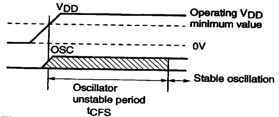
Figure 3 Oscillator Stabilization Period
