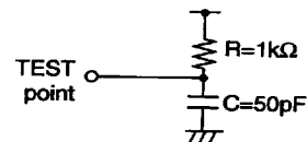
Figure 5 Timing Load
