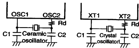
Figure 2 Ceramic Oscillator Circuit
