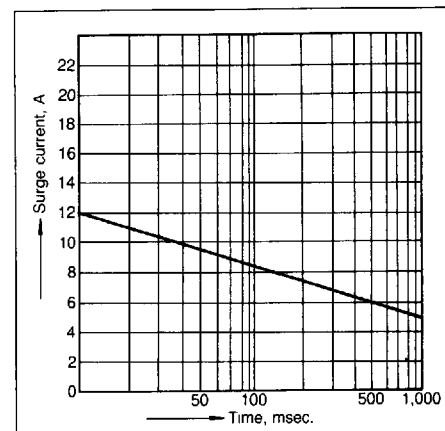
2-2. Surge current and time (IDC)
