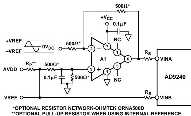
Figure 36. Single-Ended Input With DC-Coupled Level-Shift
