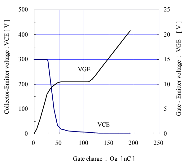
[ Brake ] Dynamic Gate charge (typ.) V_{CE} = 300\text{V} , I_C = 50\text{A} , T_j = 25^\circ\text{C}
