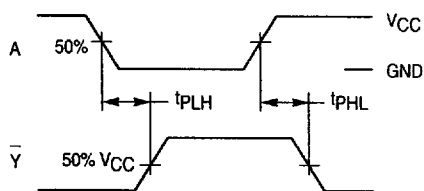
Figure 1. Switching Waveforms
