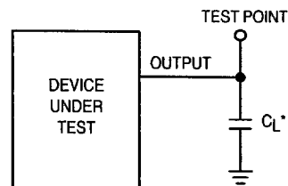
Figure 2. Test Circuit
