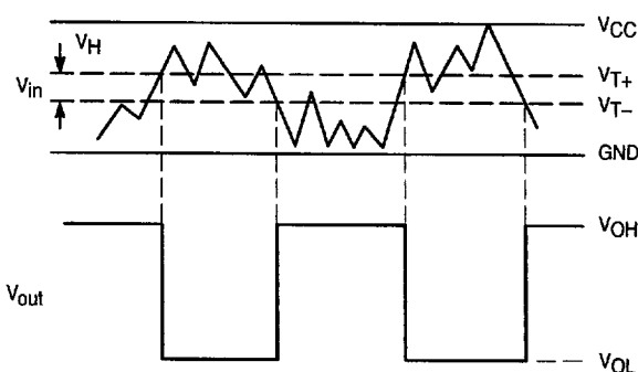
Figure 4. Typical Schmitt-Trigger Applications
