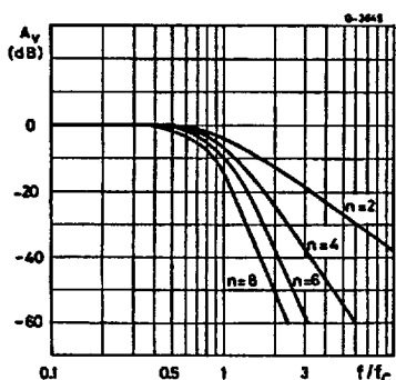
Figure 11 : Amplitude Response
