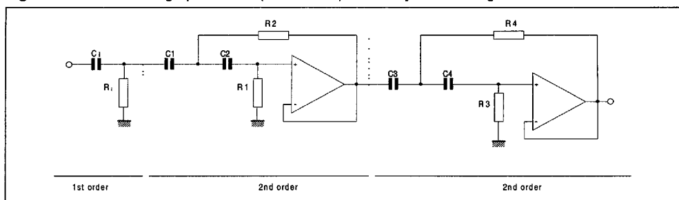
Figure 16 : 5th Order High-pass Filter (Butterworth) with Unity Gain Configuration
