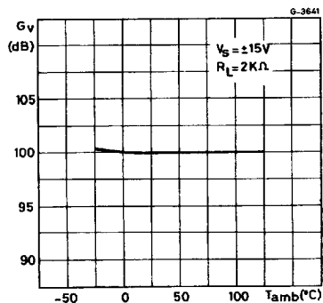
Figure 5 : Output Loop Gain versus Ambient Temperature
