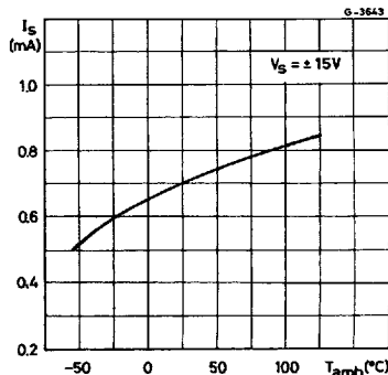
Figure 2 : Supply Current versus Ambient Temperature
