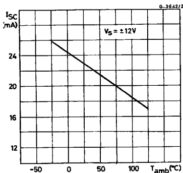
Figure 3 : Output Short Circuit Current versus Ambient Temperature
