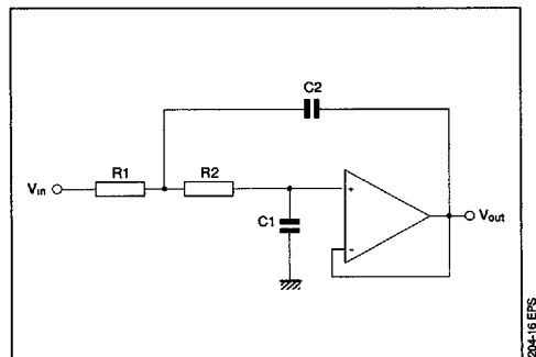
Figure 13 : Filter Configuration
