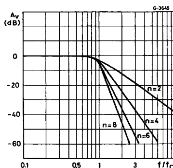
Figure 12 : Amplitude Response ( \pm 1dB ripple)
