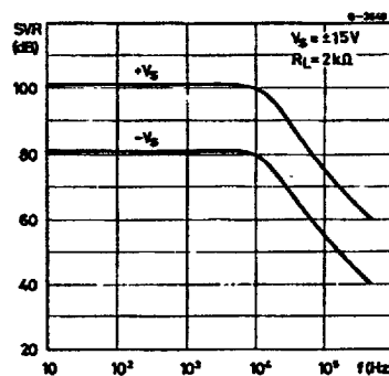
Figure 6 : Supply Voltage Rejection versus Frequency
