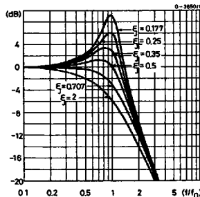
Figure 14 : Filter Respon versus Damping Factor
