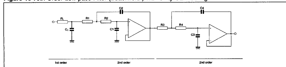
Figure 15 : 5th Order Low-pass Filter (Butterworth) with Unity Gain Configuration
