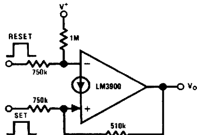
Bi-Stable Multivibrator
