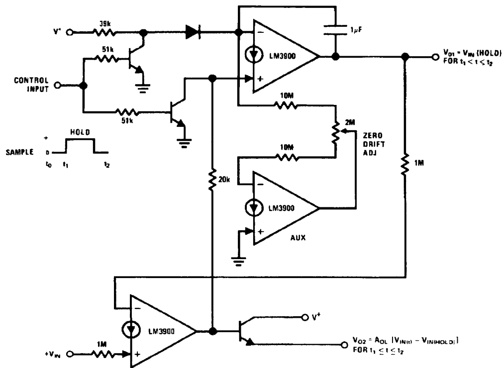
Sample-and-Hold and Compare with New +V_{\text{IN}}
