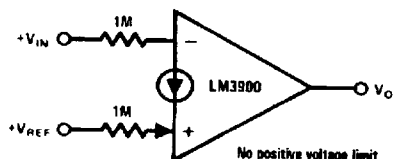
Comparator
