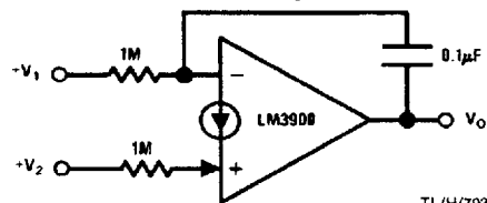
Difference Integrator
