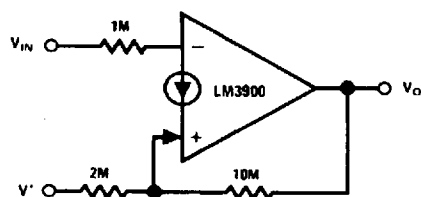
Schmitt-Trigger
