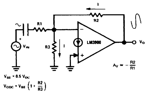
V_{\text{BE}} Biasing
