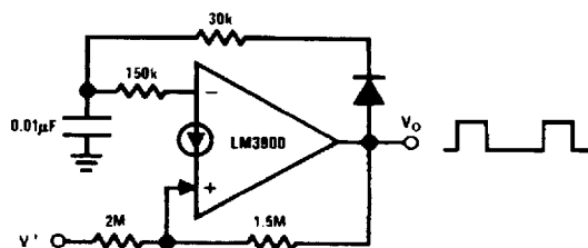
Pulse Generator
