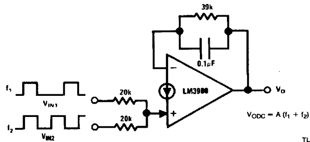
Frequency Averaging Tachometer
