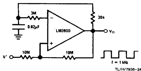
Square-Wave Oscillator
