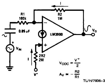
Inverting Amplifier
