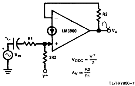
Non-Inverting Amplifier
