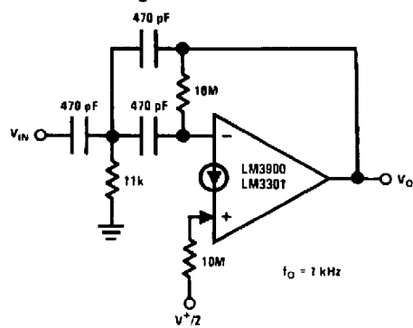
High Pass Active Filter
