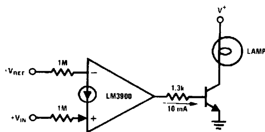
Power Comparator
