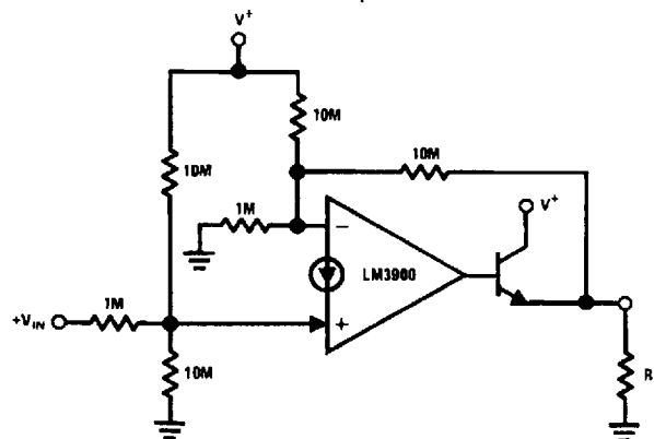
Power Amplifier
