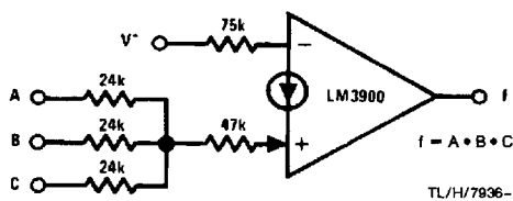
"AND" Gate
