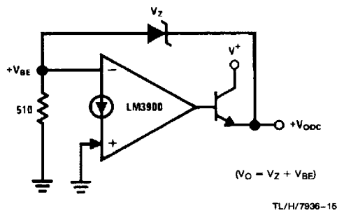
Voltage Regulator
