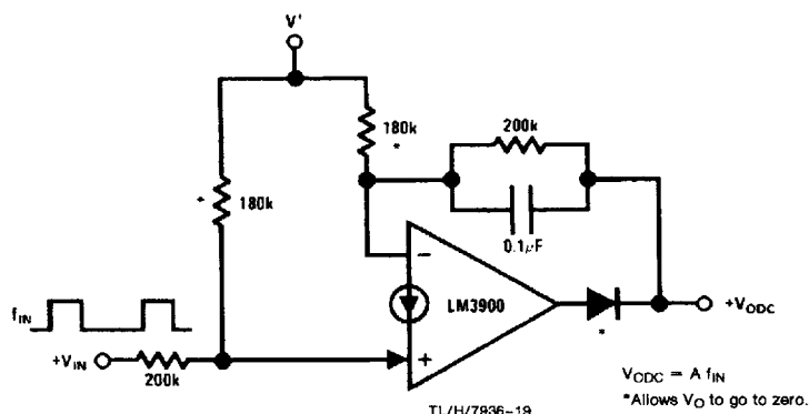
Tachometer
