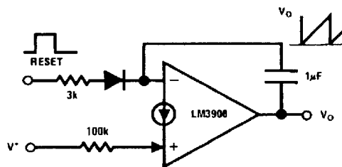
Sawtooth Generator
