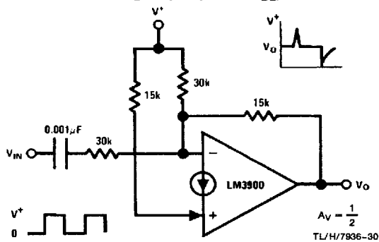
Differentiator (Common-Mode Biasing Keeps Input at +V_{BE} )
