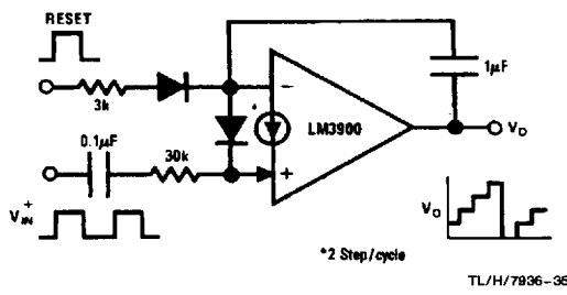
Staircase Generator
