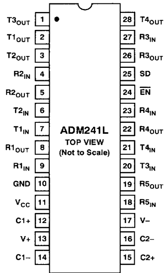
Figure 21. ADM241L SOIC/SSOP Pin Configuration
