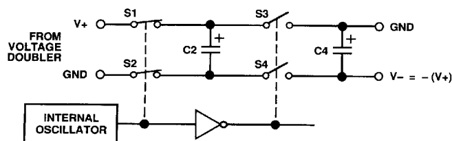
Figure 34. Charge-Pump Voltage Inverter
