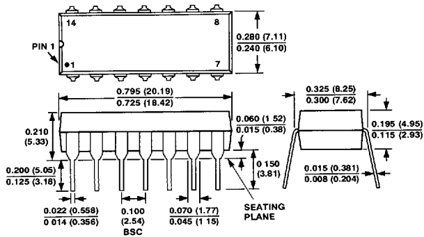
14-Lead Plastic DIP (N-14)
