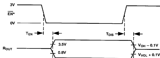
Figure 35. Enable Timing
