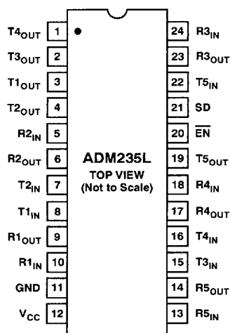
Figure 11. ADM235L DIP Pin Configuration
