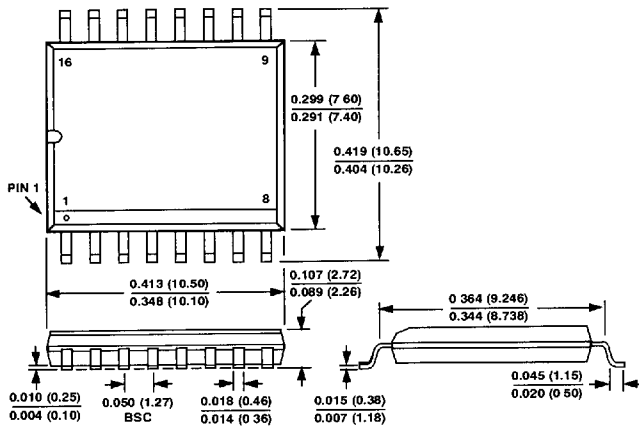
16-Lead SOIC (R-16)
