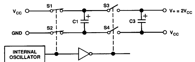
Figure 33. Charge-Pump Voltage Doubler
