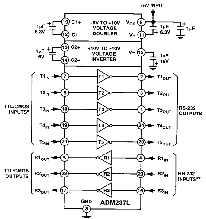
Figure 16. ADM237L Typical Operating Circuit
