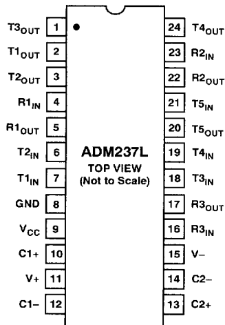
Figure 15. ADM237L DIP/SOIC Pin Configuration
