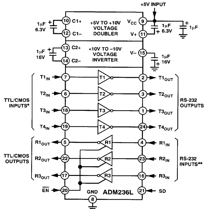
Figure 14. ADM236L Typical Operating Circuit
