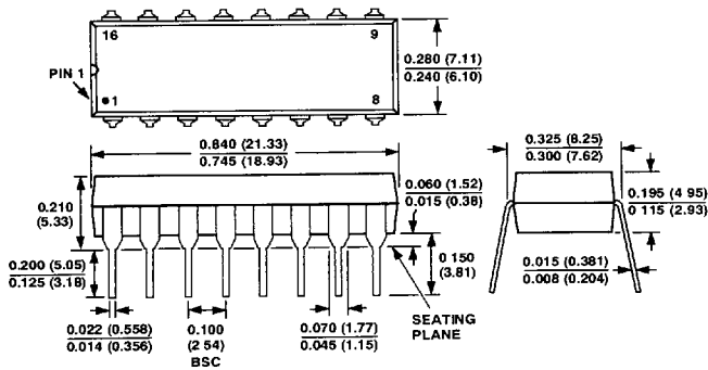
16-Lead Plastic DIP (N-16)
