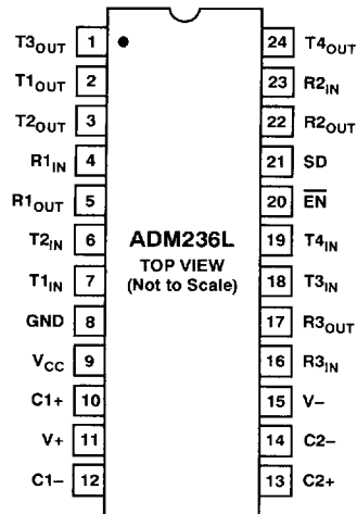
Figure 13. ADM236L DIP/SOIC Pin Configuration
