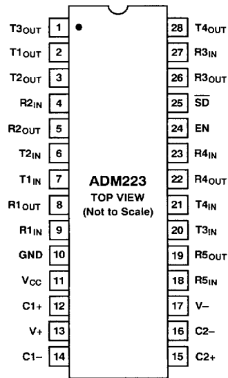
Figure 23. ADM223 SOIC/SSOP Pin Configuration
