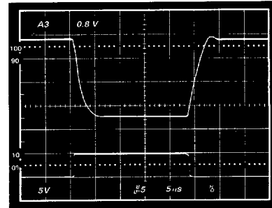
Figure 31. Transmitter Output Loaded Slew Rate
