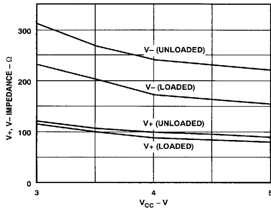
Figure 29. Charge Pump Impedance vs. V_{CC}
