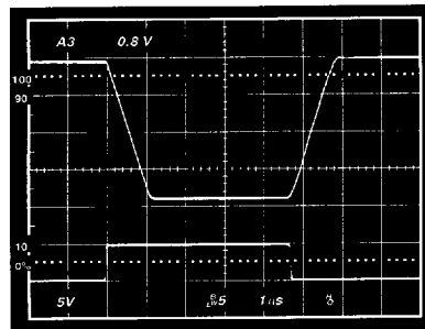
Figure 32. Transmitter Output Unloaded Slew Rate
