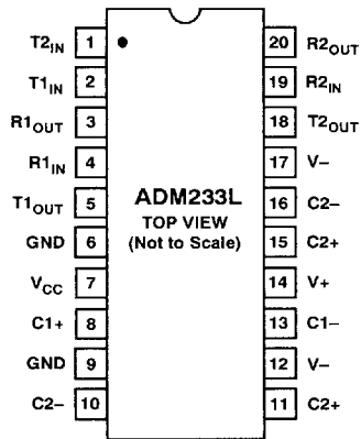
Figure 7. ADM233L DIP Pin Configuration
