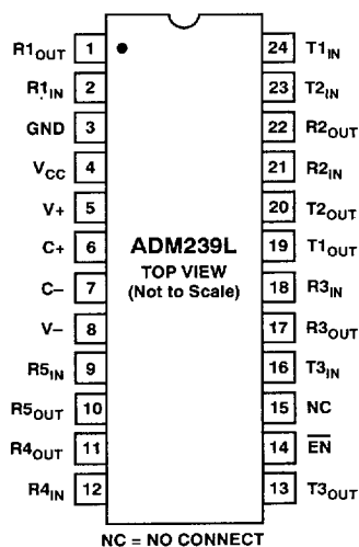
Figure 19. ADM239L DIP/SOIC Pin Configuration
