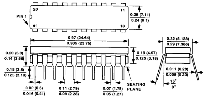
20-Lead Cerdip (Q-20)
