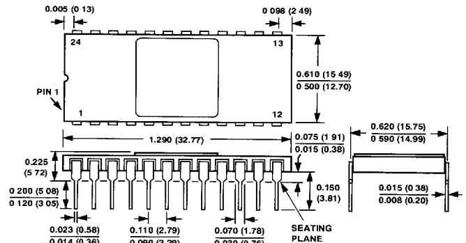
24-Lead Ceramic DIP (D-24)
