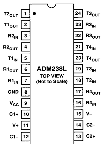
Figure 17. ADM238L DIP/SOIC Pin Configuration
