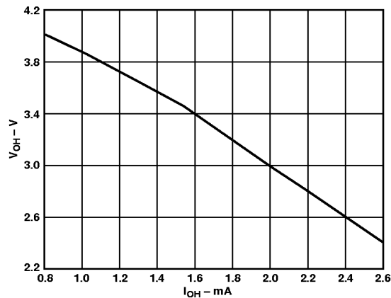
Figure 27. Source Capability of Status Output (ADD C02805SA)
