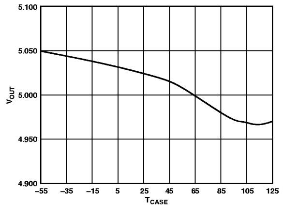
Figure 5. Output Voltage vs. Case Temperature (°C) (ADDC02805SA)
