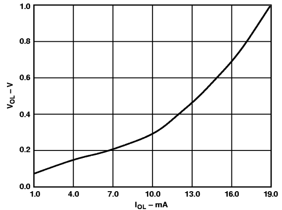
Figure 28. Sink Capability of Status Output
