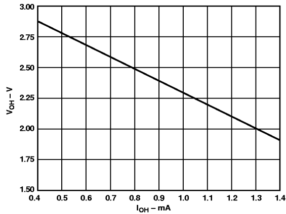
Figure 26. Source Capability of Status Output (ADD C02803SC)
