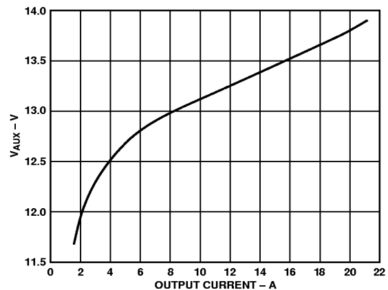
Figure 30. V_{AUX} vs. Converter Output Current (ADD C02803SC)
