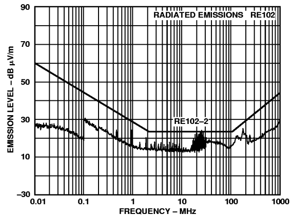
Figure 22. Radiated Emissions, MIL-STD-461D, RE102, Vertical Polarity, 100 W Load
