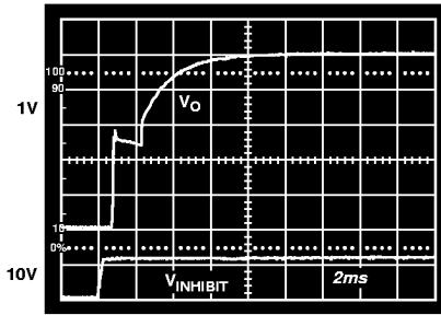
Figure 7. Output Voltage Transient During Turn-On with Minimum Load Displaying Soft Start When Supply Is Enabled (ADDC02805SA)
