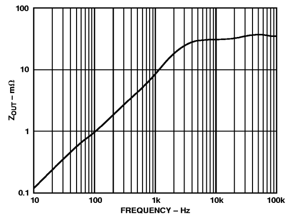
Figure 16. Incremental Output Impedance (Magnitude) (ADDC02803SC)
