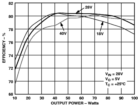
Figure 1. Efficiency vs. Line and Load at +25°C (ADDC02805SA)
