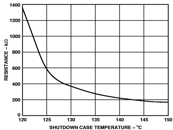
Figure 32. External Resistor Value for Raising Temperature Shutdown Point
