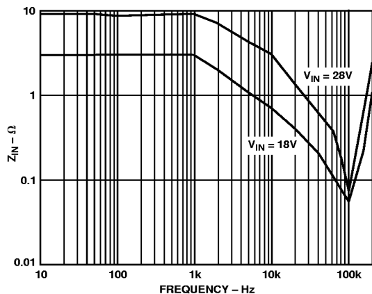
Figure 14. Incremental Input Impedance (Magnitude) (ADDC02803SC)
