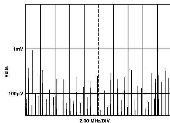
Figure 18. Output Voltage Ripple Spectrum (ADDC02805SA)
