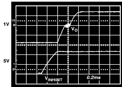
Figure 8. Output Voltage Transient During Turn-On with Minimum Load Displaying Soft Start When Supply Is Enabled (ADDC02803SC)
