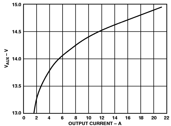
Figure 29. V_{AUX} vs. Converter Output Current (ADD C02805SA)
