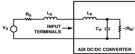
Figure 33. Model of Power Source and POL Converter Connection
