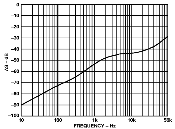
Figure 12. Audio Susceptibility (Magnitude of V_{OUT}/V_{IN} ) (ADDC02803SC)
