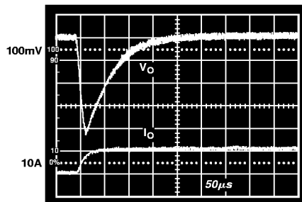
Figure 9. Output Voltage Transient Response to a 10 A to 20 A Step Change in Load with Zero Load Capacitance (ADDC02805SA)
