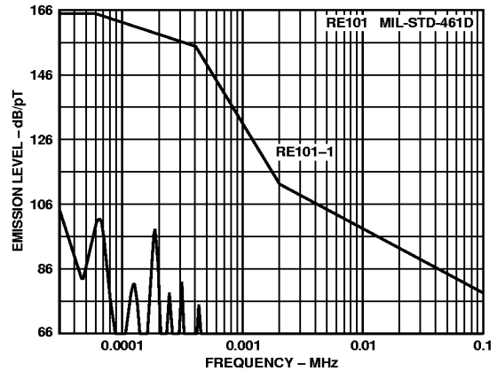
Figure 21. Radiated Emissions, MIL-STD-461D, RE101, 100 W Load
