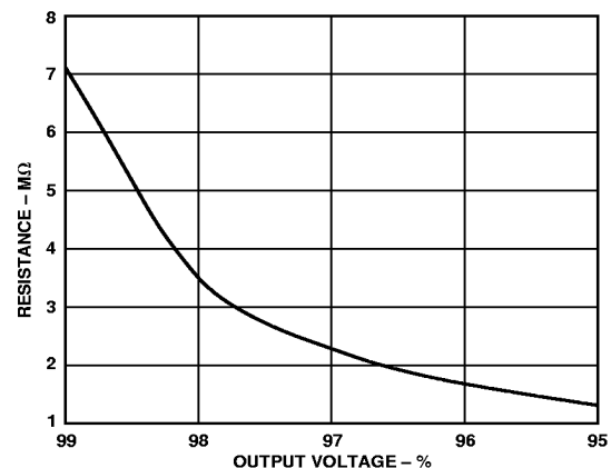
Figure 24. External Resistor Value for Reducing Output Voltage
