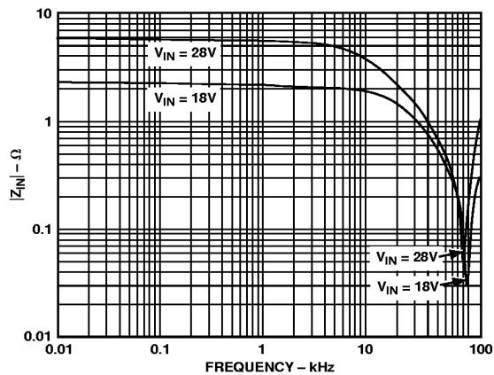
Figure 13. Incremental Input Impedance (Magnitude) (ADDC02805SA)
