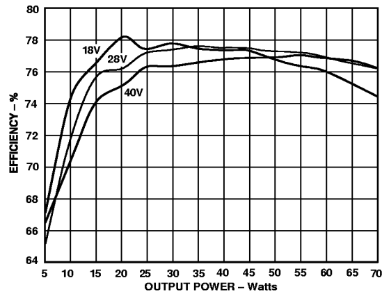
Figure 2. Efficiency vs. Line and Load at +25°C (ADDC02803SC)
