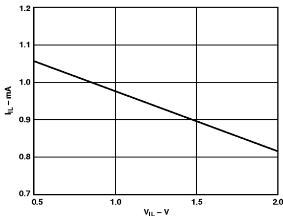
Figure 31. Input Characteristics of Pin 6 When Pulled Low
