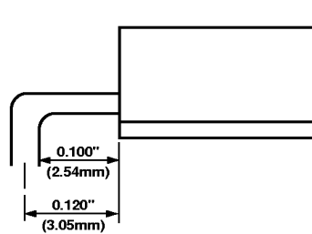
Figure 35. Minimum Bend Radius of 40 Mil (1.02 mm) Pins
