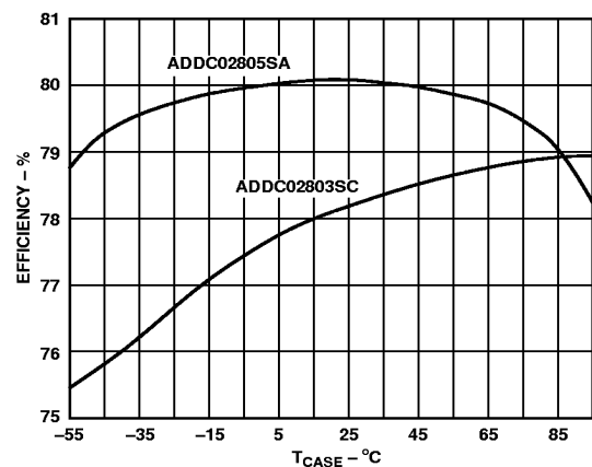
Figure 3. Efficiency vs. Case Temperature (°C) (at Nominal V_{IN} , 75% Max Load)
