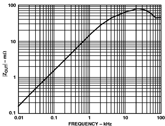
Figure 15. Incremental Output Impedance (Magnitude) (ADDC02805SA)
