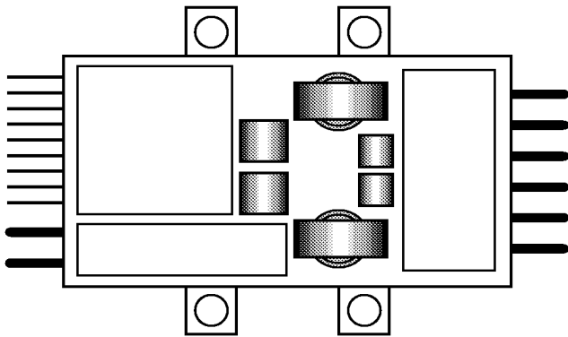
Figure 34. Hot Spots (Shaded Areas) of DC/DC Converter
