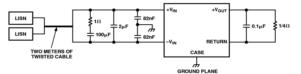
Figure 23. Schematic of Test Setup for EMI Measurements
