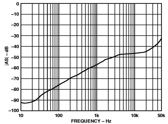
Figure 11. Audio Susceptibility (Magnitude of V_{OUT}/V_{IN} ) (ADDC02805SA)
