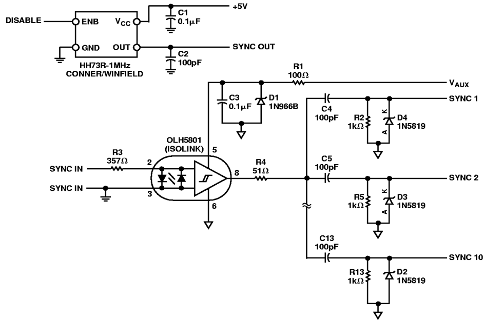
Figure 38. Fault Tolerant, Secondary Side Powered SYNC Drive Circuit
