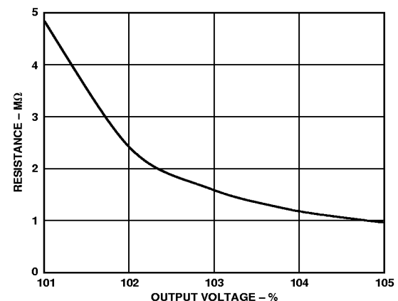
Figure 25. External Resistor for Increasing Output Voltage
